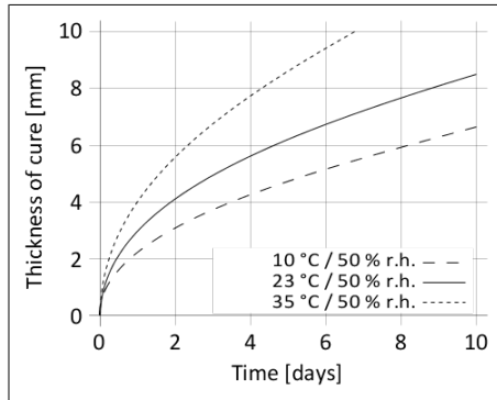
Diagram 1: Curing speed Sikaflex®-554
