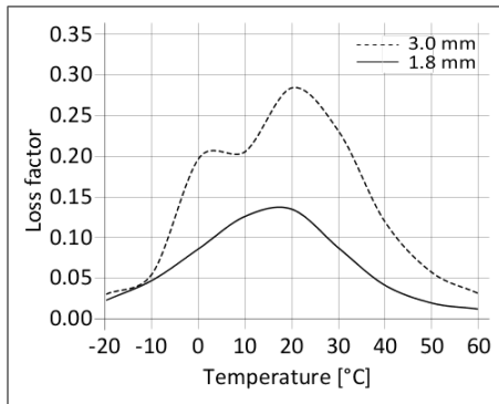
Diagram 1: Loss factor SikaDamp®-115 at 200 Hz
