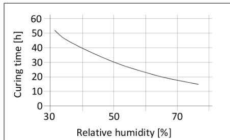
Diagram 1: Curing time for 500 µm film
