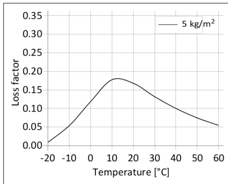
Diagram 1: Loss factor SikaDamp®-140 AL at 200 Hz
