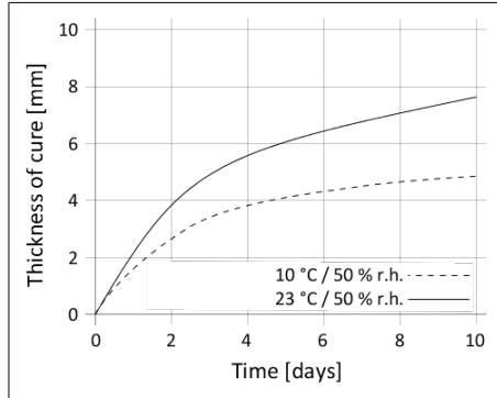
Diagram 1: Curing speed Sikaflex®-529 Evolution
