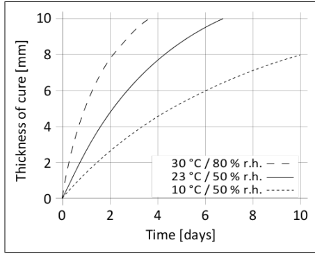
Diagram 1: Curing speed Sikaflex®-268
