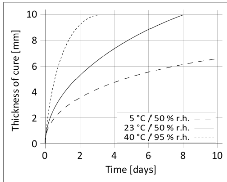
Diagram 1: Curing speed Sikasil® WS-605 S
