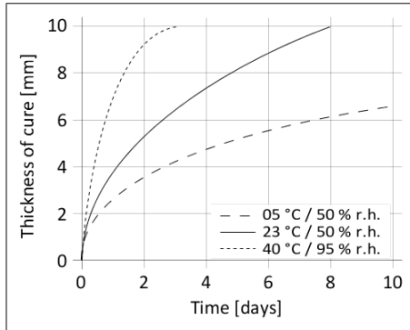
Diagram 1: Curing speed Sikasil® WS-305 EU
