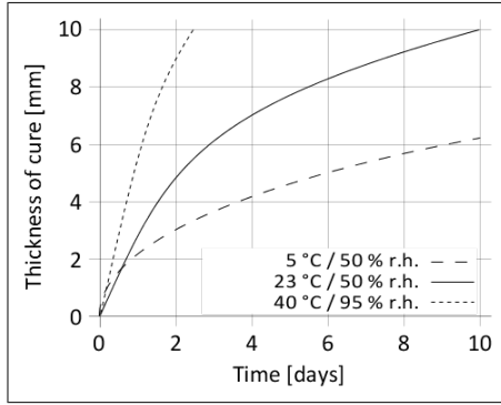
Diagram 1: Curing speed Sikasil® SG-20 S
