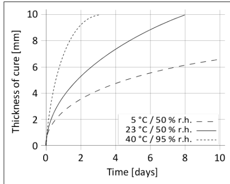
Diagram 1: Curing speed Sikasil® WS-305 EU
