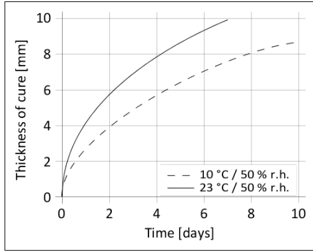
Diagram 1: Curing speed of SikaTack® MOVE Transportation
