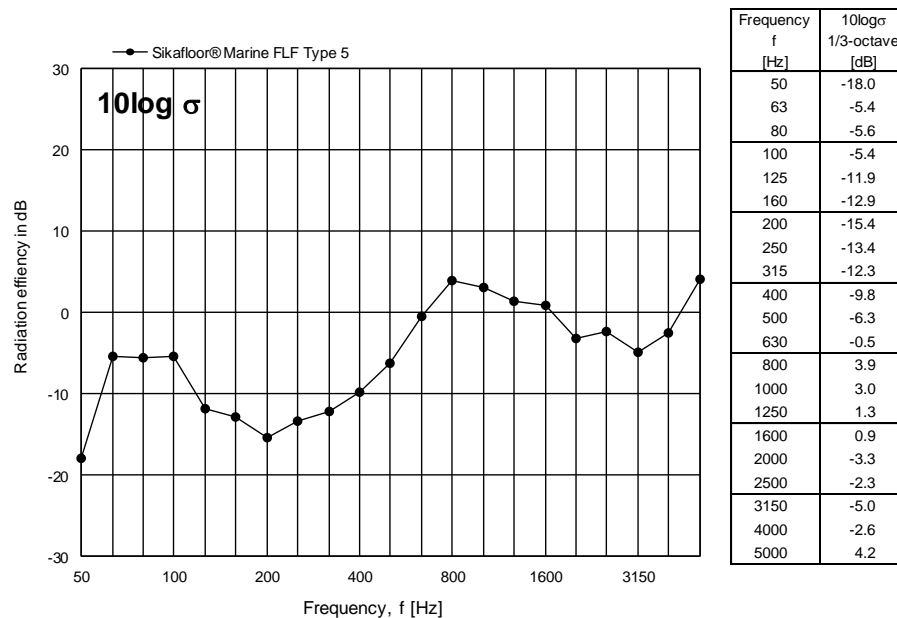
Figure 9 Measured radiation index 10 \log \sigma for Sikafloor® Marine FLF Type 5 expressed in dB per one-third octave frequency band.
