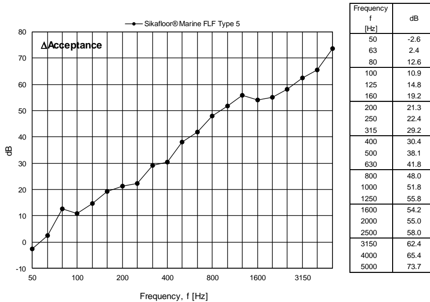
Figure 14 Measured change in acceptance for Sikafloor® Marine FLF Type 5 expressed in dB per one-third octave frequency band.
