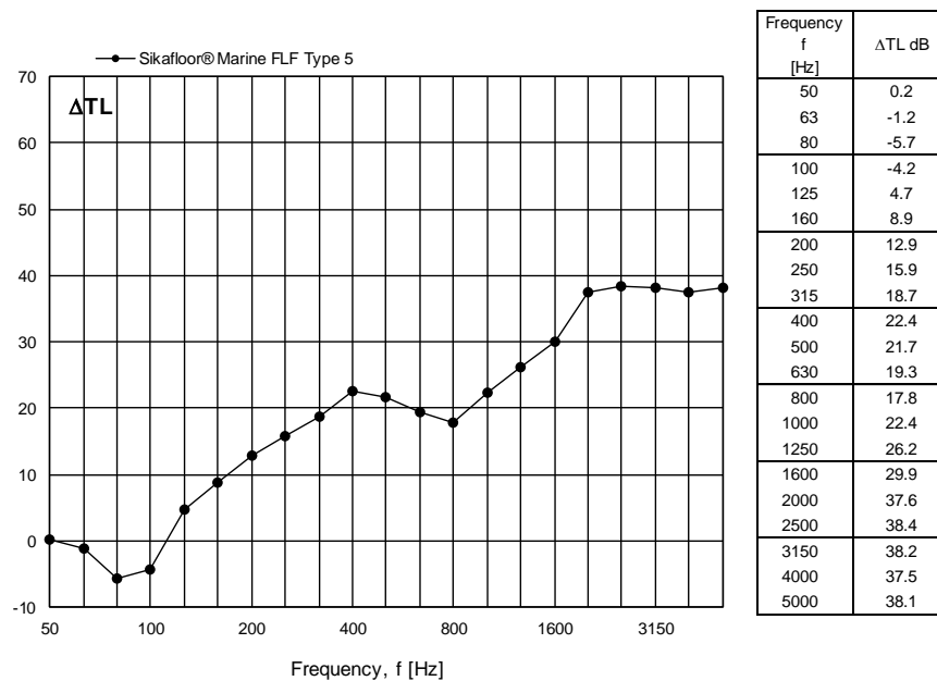
Figure 13 Measured changes in transmission loss TL for Sikafloor® Marine FLF Type 5 expressed in dB per one-third octave frequency band.
