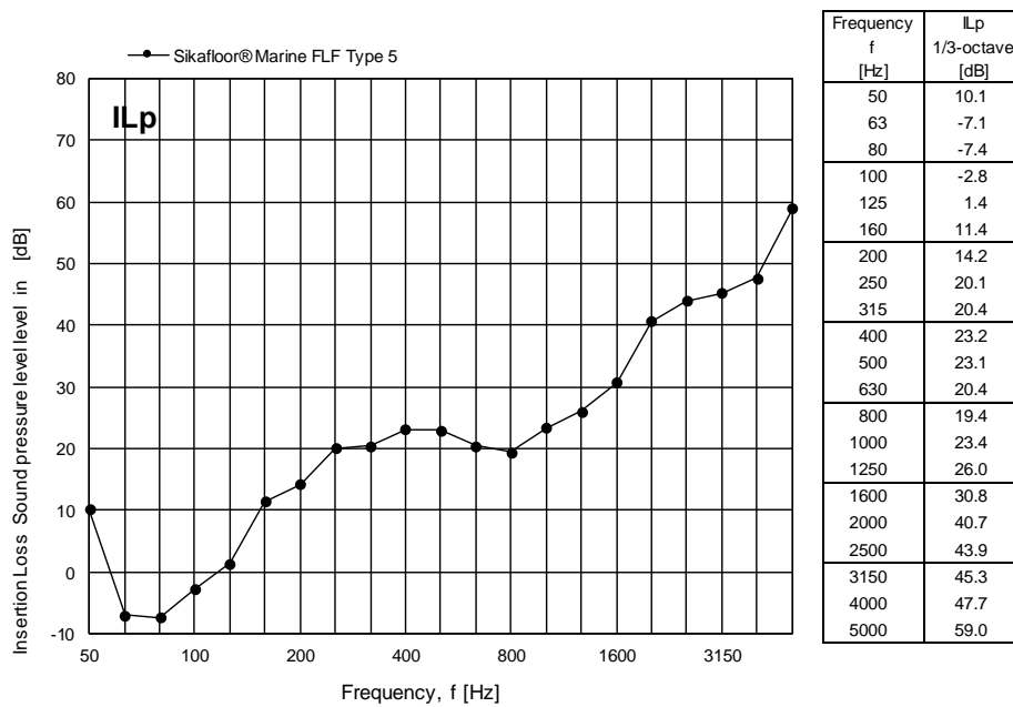
Figure 8 Measured insertion loss IL_p for Sikafloor® Marine FLF Type 5 expressed in dB per one-third octave frequency band. The insertion loss IL_p refers to the radiated mean sound pressure level in dB re 20 \mu Pa in the receiving room above the floor.
