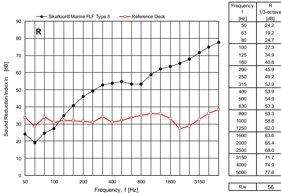
Figure 4 Measured sound reduction index R for the Sikafloor® Marine FLF Type 5 expressed in dB per one-third octave frequency bands. For comparison the results of the measurements on the bare steel deck are also shown.
