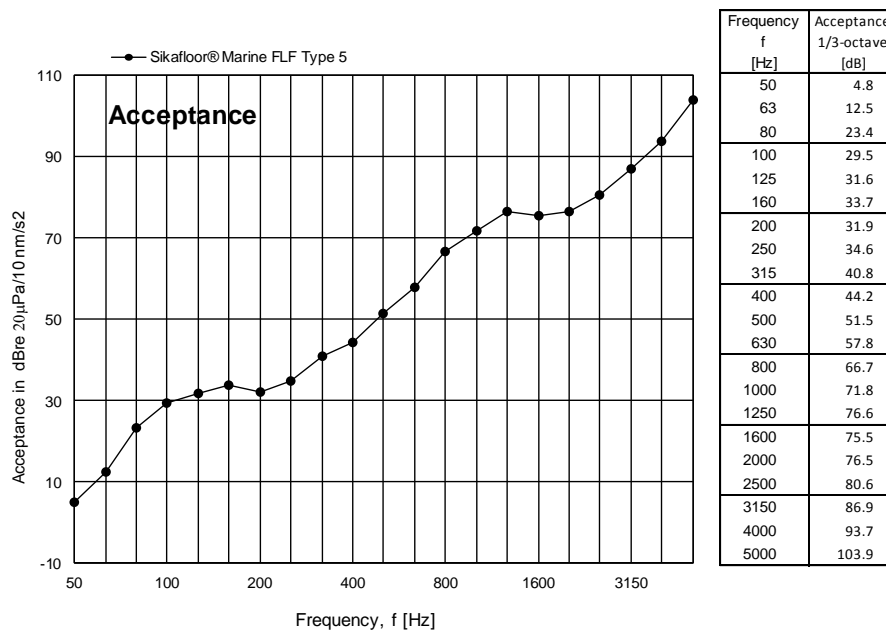
Figure 11 Measured acceptance LA for Sikafloor® Marine FLF Type 5 expressed in dB per one-third octave frequency band.
