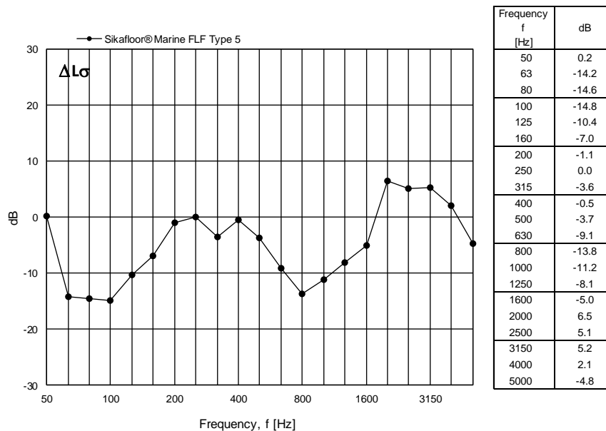
Figure 15 Measured change in radiation efficiency for Sikafloor® Marine FLF Type 5 expressed in dB per one-third octave frequency band.
