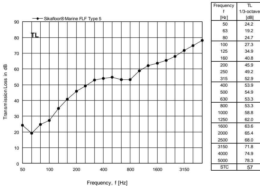
Figure 10 Measured transmission loss TL for Sikafloor® Marine FLF Type 5 expressed in dB per one-third octave frequency band.
