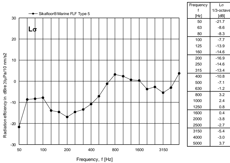
Figure 12 Measured radiation index L_{\sigma} for Sikafloor® Marine FLF Type 5 expressed in dB per one-third octave frequency band.
