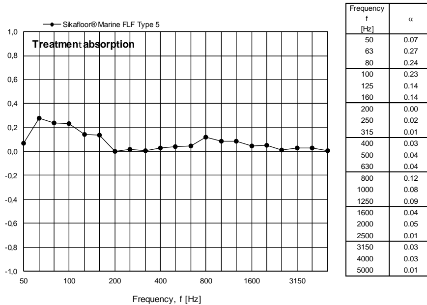
Figure 16 Measured treatment absorption for Sika floor® Marine FLF Type 5 per one-third octave frequency band.
