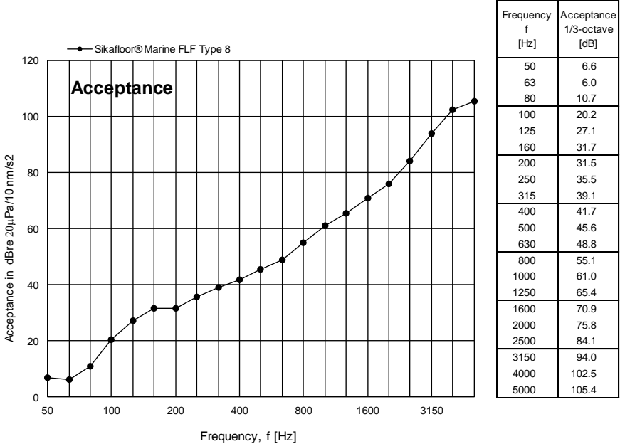
Figure 11 Measured acceptance LA for Sikafloor® Marine FLF Type 8 expressed in dB per one-third octave frequency band.
