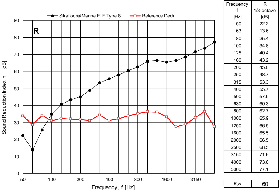
Figure 4 Measured sound reduction index R for the Sika floor® Marine FLF Type 8 expressed in dB per one-third octave frequency bands. For comparison the results of the measurements on the bare steel deck are also shown.
