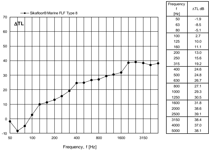
Figure 13 Measured changes in transmission loss TL for Sikafloor® Marine FLF Type 8 expressed in dB per one-third octave frequency band.
