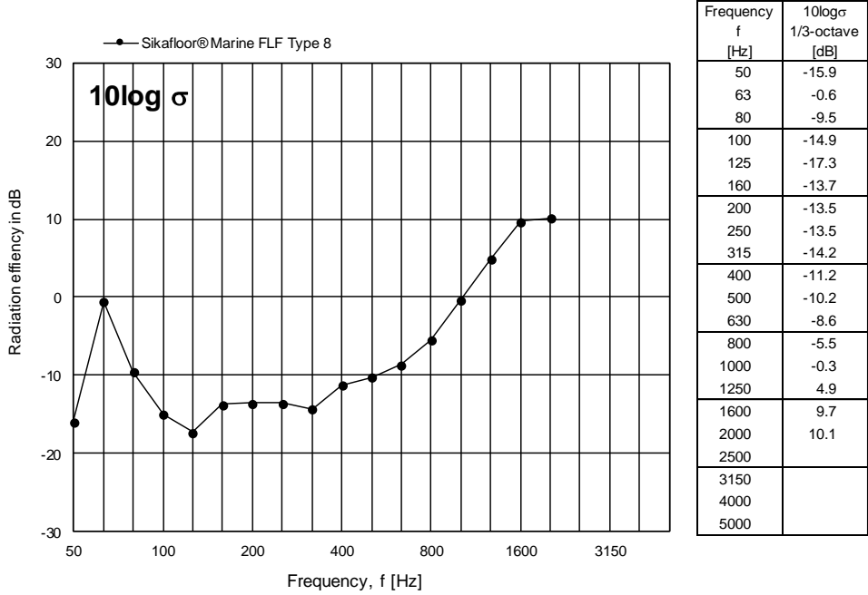
Figure 9 Measured radiation index 10 \log \sigma for Sikafloor® Marine FLF Type 8 expressed in dB per one-third octave frequency band.
