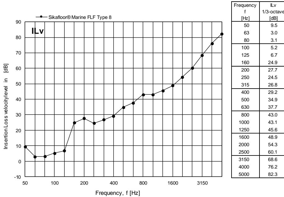
Figure 6 Measured Insertion Loss IL_v for Sikafloor® Marine FLF Type 8 expressed in dB per one-third octave frequency band. The insertion loss IL_v refers to the mean velocity level in dB re 10 -9 m/s on top of the floor covering.
