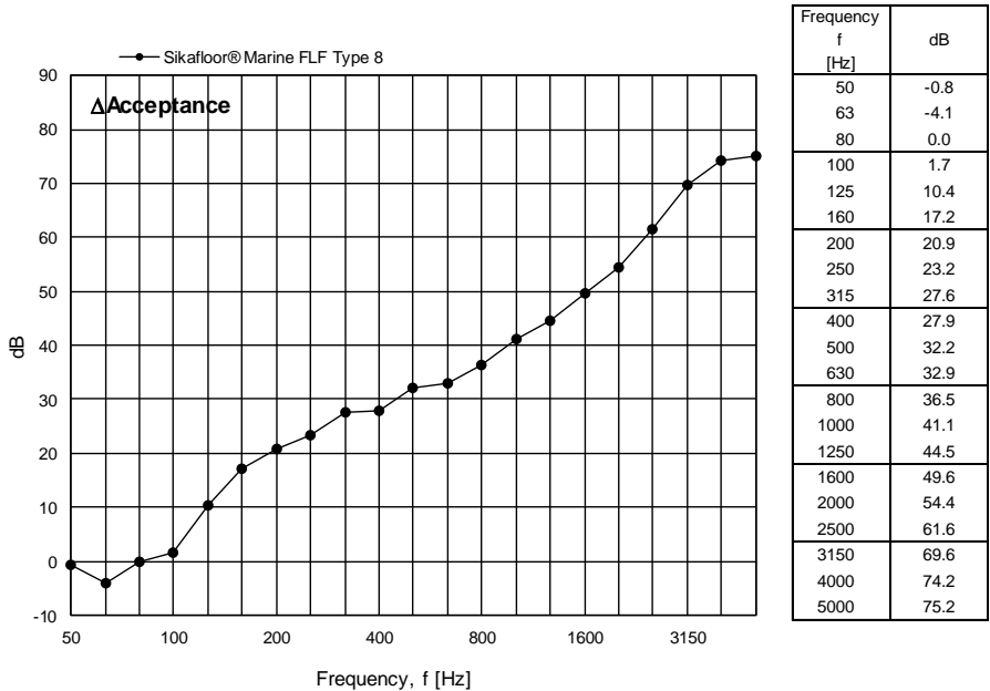
Figure 14 Measured change in acceptance for Sikafloor® Marine FLF Type 8 expressed in dB per one-third octave frequency band.
