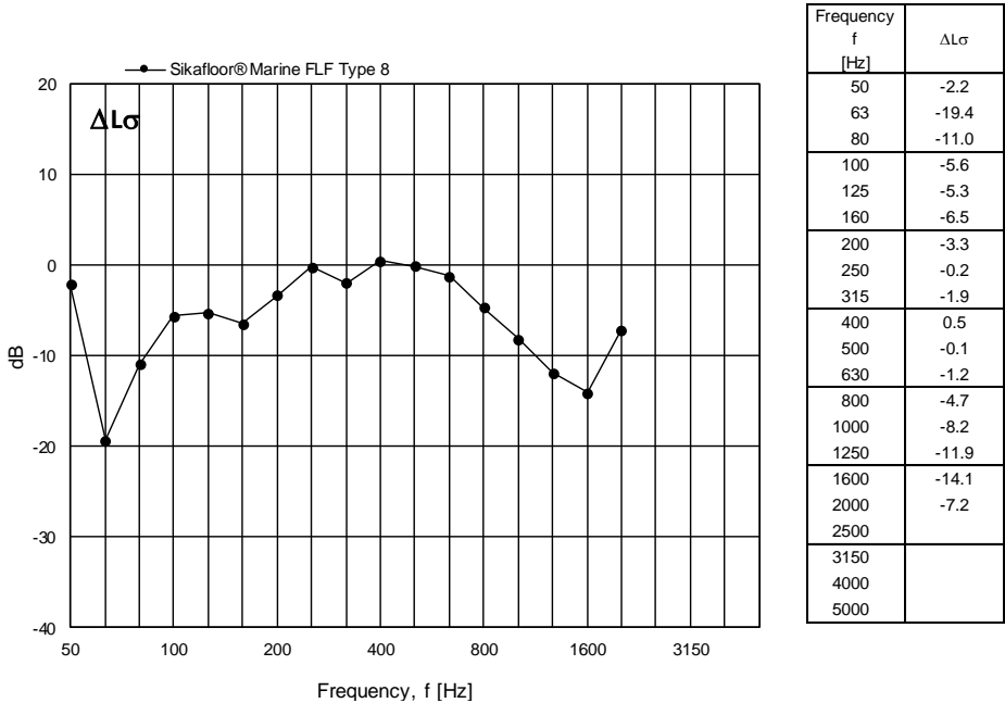
Figure 15 Measured change in radiation efficiency for Sikafloor® Marine FLF Type 8 expressed in dB per one-third octave frequency band.
