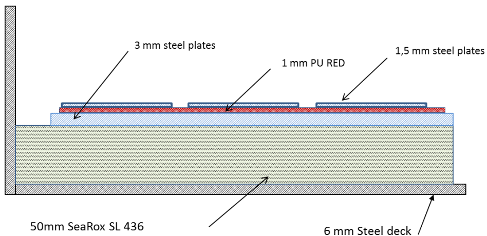
Figure 3 Principle sketch of the test construction.
