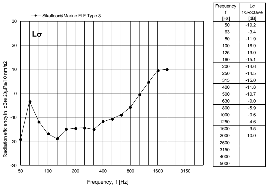
Figure 12 Measured radiation index L_{\sigma} for Sikafloor® Marine FLF Type 8 expressed in dB per one-third octave frequency band.
