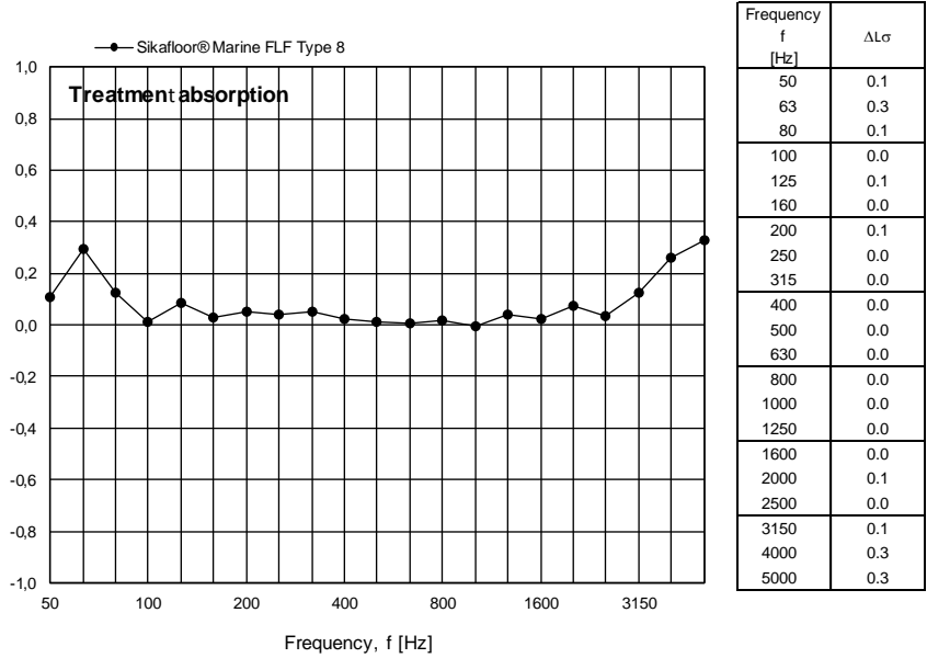
Figure 16 Measured treatment absorption for Sikafloor® Marine FLF Type 8 per one-third octave frequency band.
