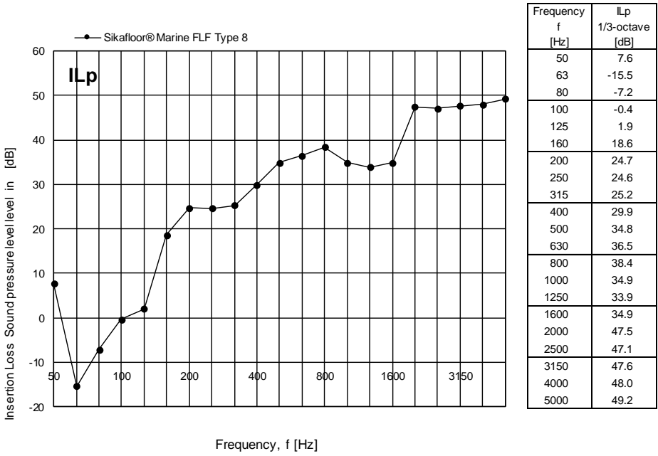
Figure 8 Measured insertion loss IL_p for Sikafloor® Marine FLF Type 8 expressed in dB per one-third octave frequency band. The insertion loss IL_p refers to the radiated mean sound pressure level in dB re 20 \mu Pa in the receiving room above the floor.
