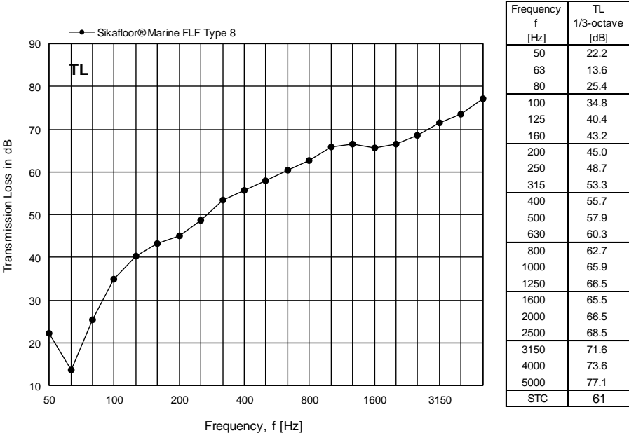
Figure 10 Measured transmission loss TL for Sikafloor® Marine FLF Type 8 expressed in dB per one-third octave frequency band.
