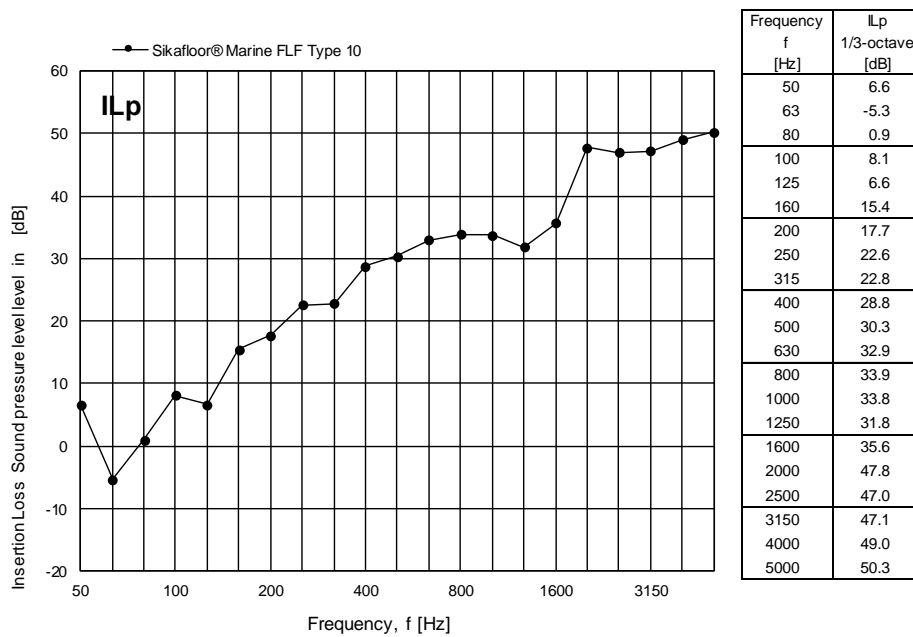
Figure 8 Measured insertion loss IL_p for Sika floor® Marine FLF Type 10 expressed in dB per one-third octave frequency band. The insertion loss IL_p refers to the radiated mean sound pressure level in dB re 20 \mu Pa in the receiving room above the floor.
