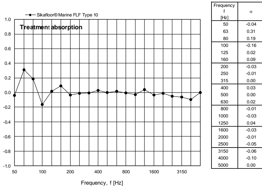
Figure 14 Measured treatment absorption for Sikafloor® Marine FLF Type 10 per one-third octave frequency band.
