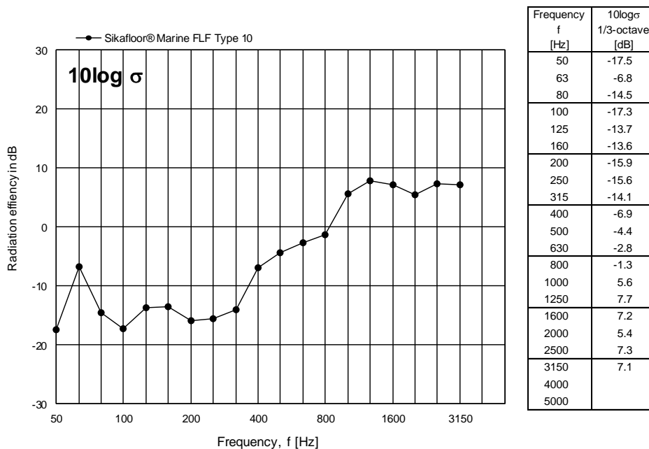
Figure 9 Measured radiation index 10 \log \sigma for Sika floor® Marine FLF Type 10 expressed in dB per one-third octave frequency band.
