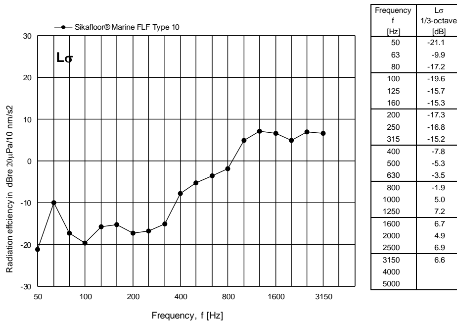
Figure 11 Measured radiation index L_{\sigma} for Sikafloor® Marine FLF Type 10 expressed in dB per one-third octave frequency band.
