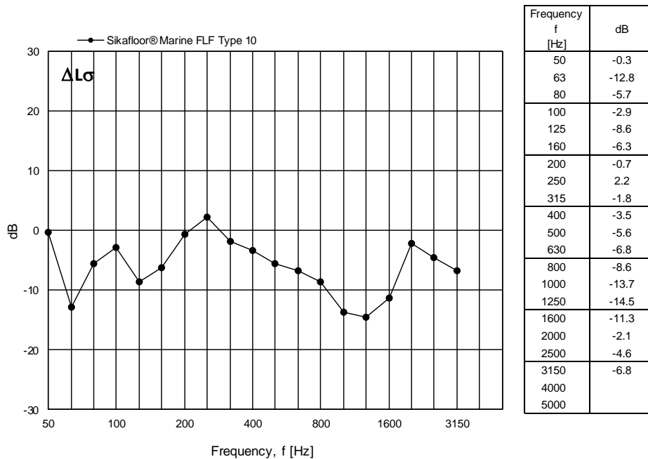
Figure 13 Measured change in radiation efficiency for Sikafloor® Marine FLF Type 10 expressed in dB per one-third octave frequency band.
