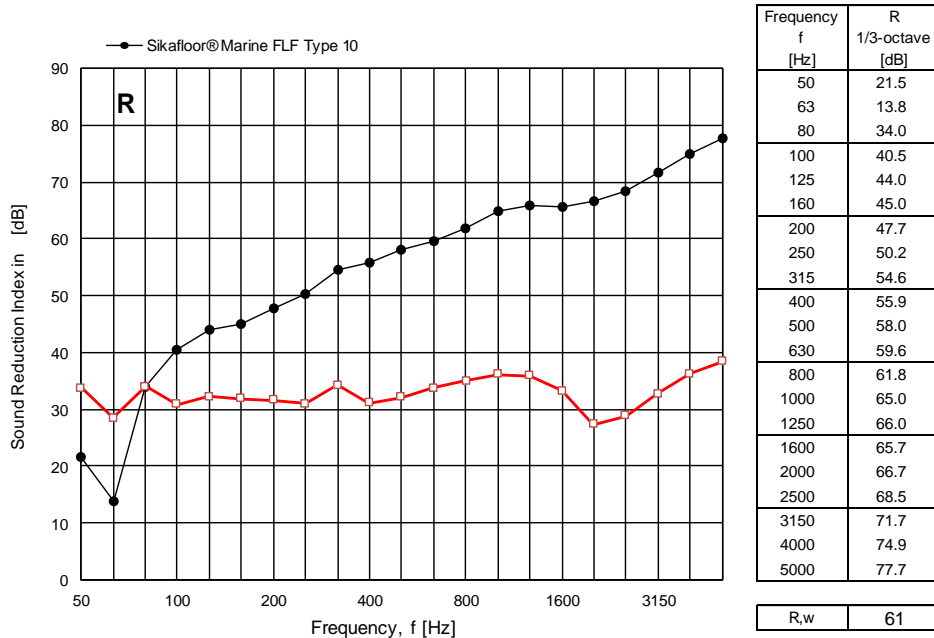
Figure 4 Measured sound reduction index R for the Sikafloor® Marine FLF Type 10 expressed in dB per one-third octave frequency bands. For comparison the results of the measurements on the bare steel deck are also shown.
