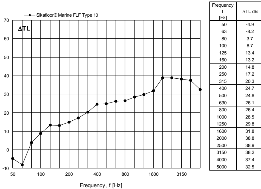
Figure 12 Measured changes in transmission loss TL for Sikafloor® Marine FLF Type 10 expressed in dB per one-third octave frequency band.
