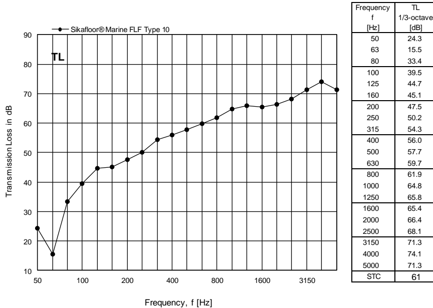
Figure 10 Measured transmission loss TL for Sikafloor® Marine FLF Type 10 expressed in dB per one-third octave frequency band.
