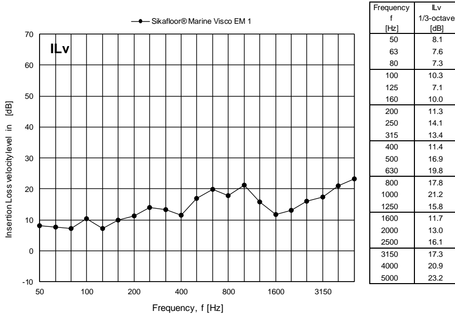
Figure 6 Measured Insertion Loss IL_v for Sikafloor® Marine Visco EM 1 expressed in dB per one-third octave frequency band. The insertion loss IL_v refers to the mean velocity level in dB re 10 -9 m/s on top of the floor covering.
