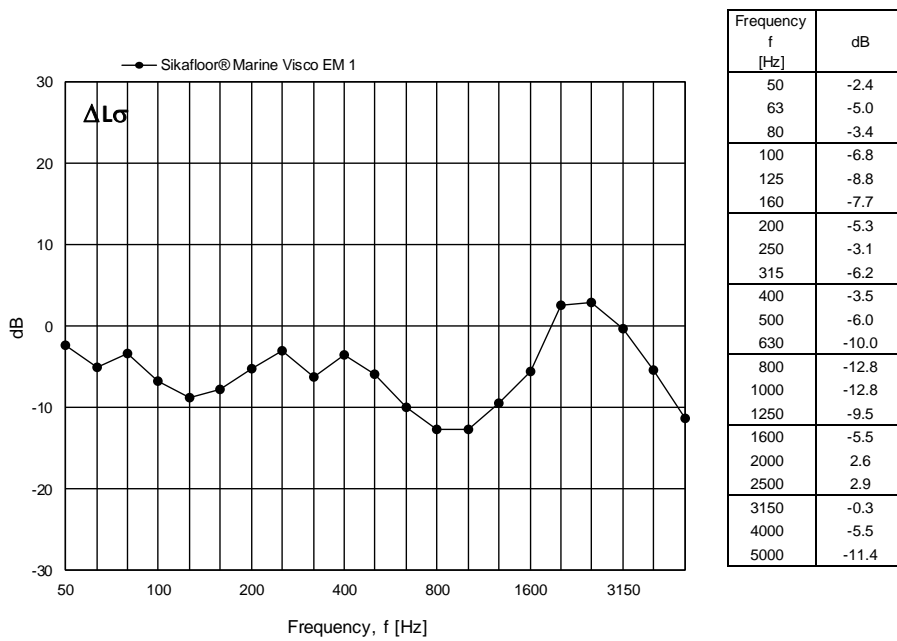
Figure 16 Measured change in radiation efficiency for Sikafloor® Marine Visco EM 1 expressed in dB per one-third octave frequency band.
