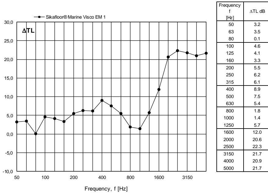
Figure 14 Measured changes in transmission loss TL for Sikafloor® Marine Visco EM 1 expressed in dB per one-third octave frequency band.
