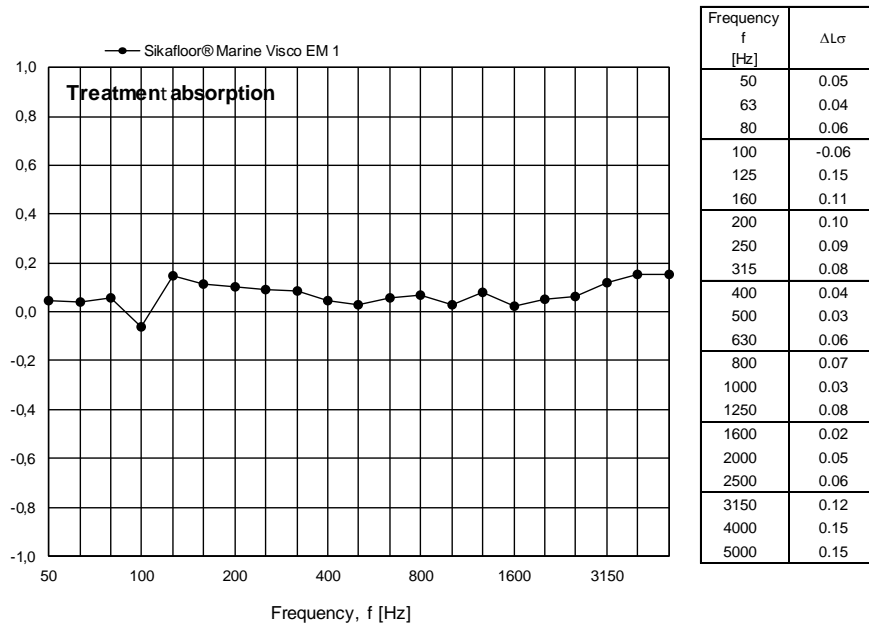
Figure 18 Measured treatment absorption for SikaFloor® Marine Visco EM 1 per one-third octave frequency band.
