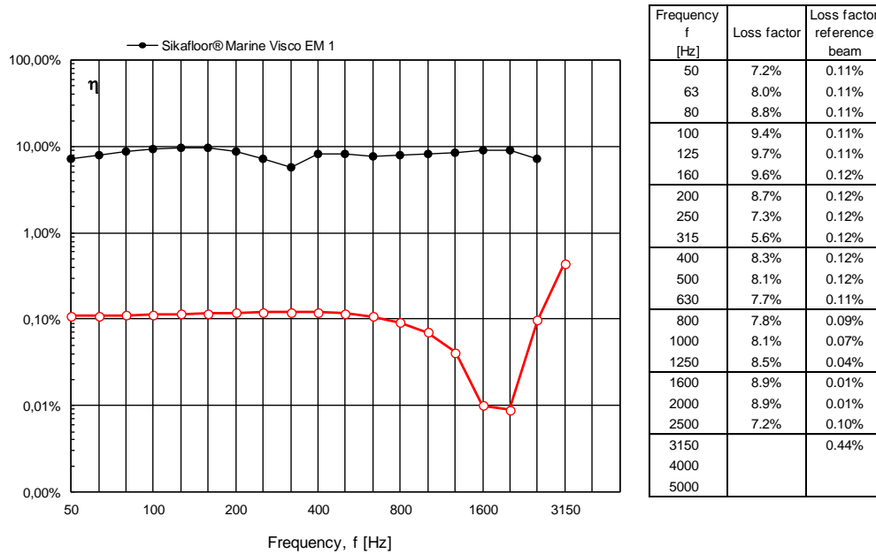
Figure 12 Measured loss factor for test beam applied with constrained damped construction type Sikafloor® Marine Visco EM 1 in % per one-third octave frequency band. For comparison the results of the measurements on a bare 6 mm steel bar are also shown.
