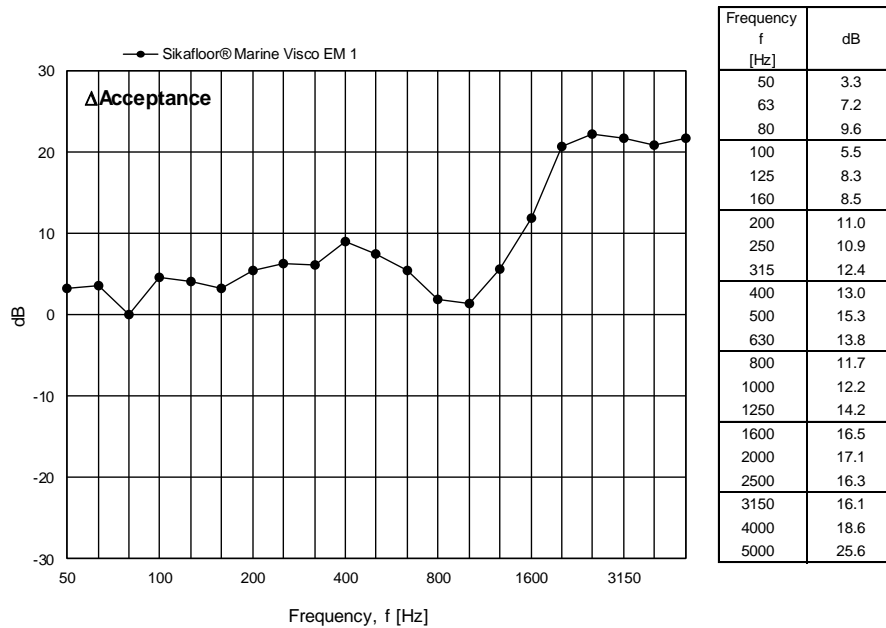
Figure 15 Measured change in acceptance for Sikafloor® Marine Visco EM 1 expressed in dB per one-third octave frequency band.
