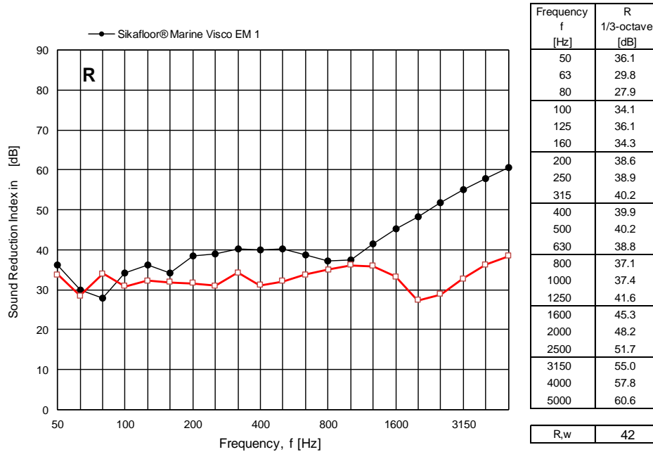
Figure 4 Measured sound reduction index R for the Sikafloor® Marine Visco EM 1 expressed in dB per one-third octave frequency bands. For comparison the results of the measurements on the bare steel deck are also shown.
