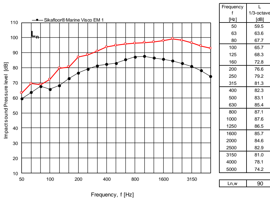
Figure 5 Measured normalized impact sound pressure level L_n for Sikafloor® Marine Visco EM 1 expressed in dB re 20 \mu Pa per one-third octave frequency band. For comparison the results of the measurements on the bare steel deck are also shown.
