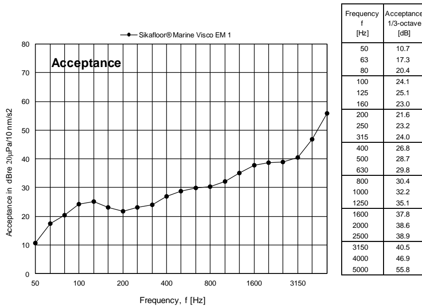
Figure 10 Measured acceptance L_A for Sikafloor® Marine Visco EM 1 expressed in dB per one-third octave frequency band.
