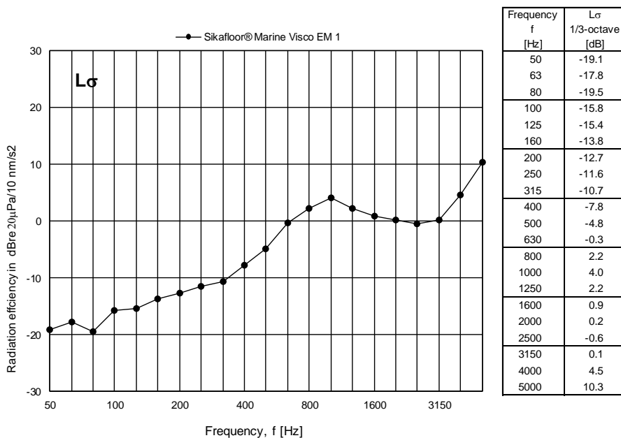
Figure 11 Measured radiation index L_\sigma for Sikafloor® Marine Visco EM 1 expressed in dB per one-third octave frequency band.
