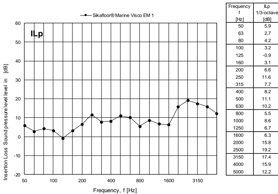
Figure 7 Measured insertion loss IL_p for Sikafloor® Marine Visco EM 1 expressed in dB per one-third octave frequency band. The insertion loss IL_p refers to the radiated mean sound pressure level in dB re 20 \mu Pa in the receiving room above the floor.
