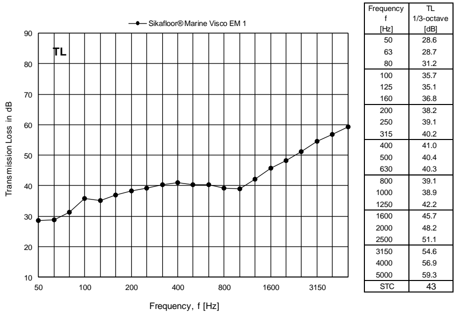
Figure 9 Measured transmission loss TL for Sikafloor® Marine Visco EM 1 expressed in dB per one-third octave frequency band.
