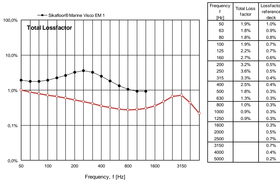
Figure 13 Measured total loss factor for test deck applied with constrained damped construction type Sikafloor® Marine Visco EM 1 in % per one-third octave frequency band. For comparison the results of the measurements on the bare 6 mm steel deck are also shown.
