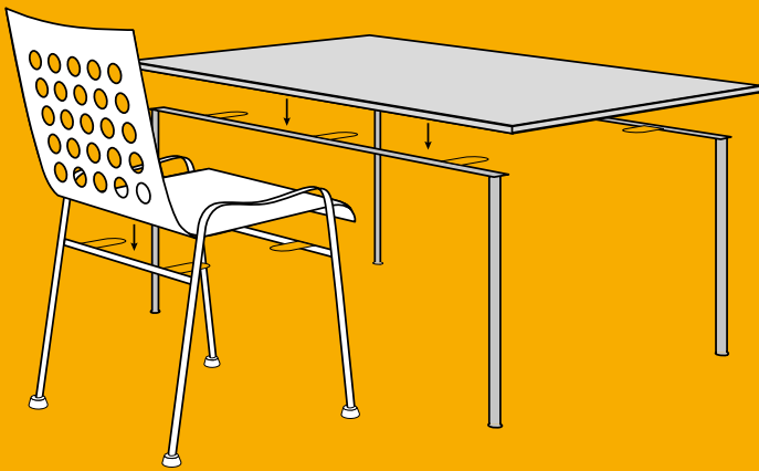
Structural bonding of seat and table on mountings with SikaFast®-555 L10 .
