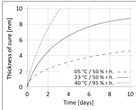
Diagram 1: Curing speed Sikasil® AS-75
