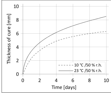
Diagram 1: Curing speed Sikaflex®-552 AT
