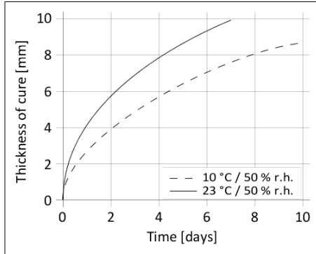
Diagram 1: curing speed Sikaflex®-255 Ultra
