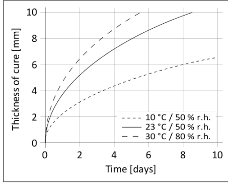
Diagram 1: Curing speed Sikaflex®-254
