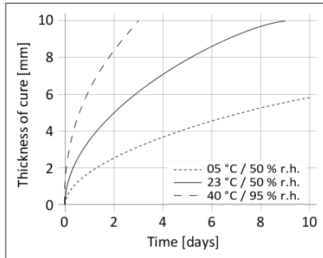
Diagram 1: Curing speed Sikasil® WS-355 N
