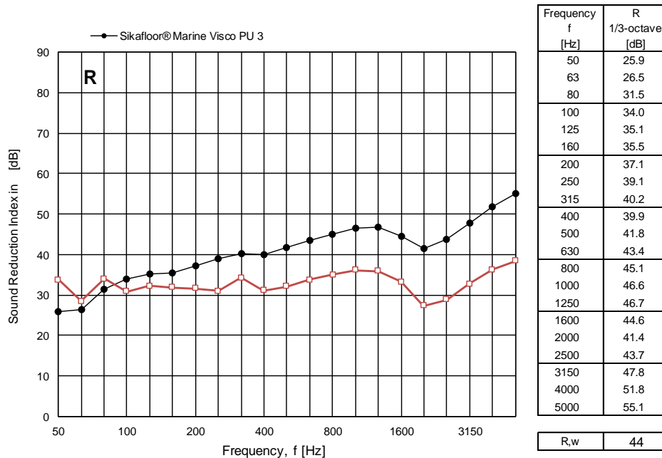
Figure 4 Measured sound reduction index R for the SikaFloor® Marine Visco PU 3 expressed in dB per one-third octave frequency bands. For comparison the results of the measurements on the bare steel deck are also shown.
