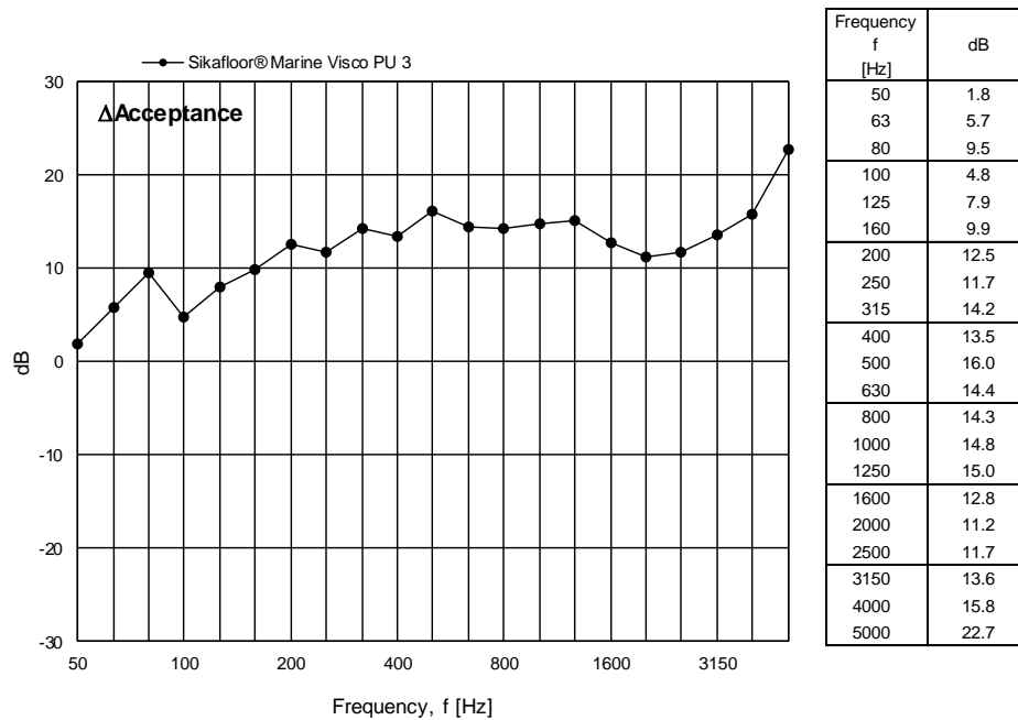
Figure 15 Measured change in acceptance for Sikafloor® Marine Visco PU 3 expressed in dB per one-third octave frequency band.
