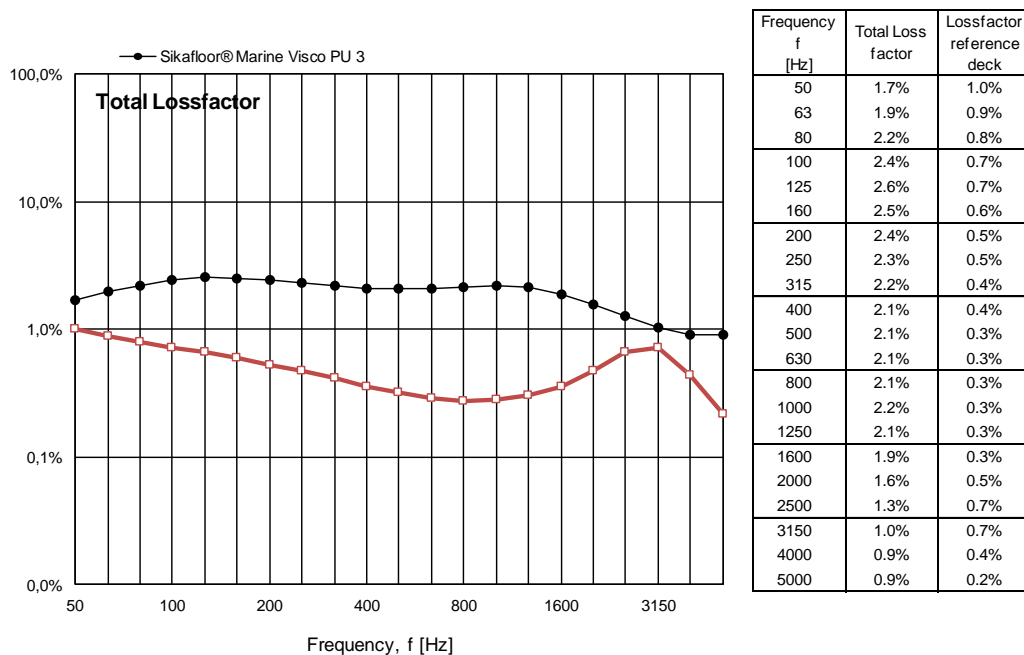
Figure 13 Measured total loss factor for test deck applied with constrained damped construction type Sikafloor® Marine Visco PU 3 in % per one-third octave frequency band. For comparison the results of the measurements on the bare 6 mm steel deck are also shown.
