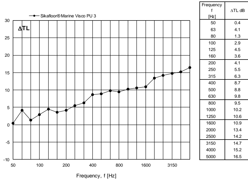
Figure 14 Measured changes in transmission loss TL for Sikafloor® Marine Visco PU 3 expressed in dB per one-third octave frequency band.
