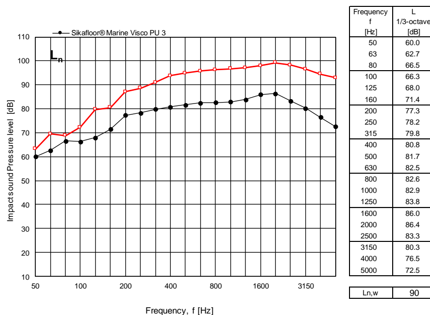
Figure 5 Measured normalized impact sound pressure level L_n for SikaFloor® Marine Visco PU 3 expressed in dB re 20 \mu Pa per one-third octave frequency band. For comparison the results of the measurements on the bare steel deck are also shown.
