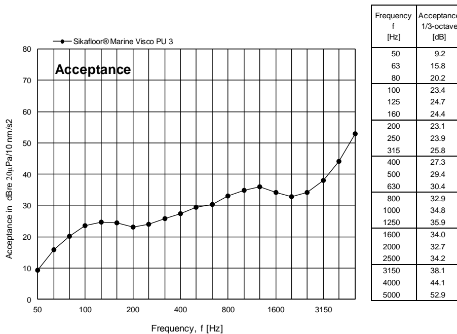
Figure 10 Measured acceptance L_A for Sikafloor® Marine Visco PU 3 expressed in dB per one-third octave frequency band.
