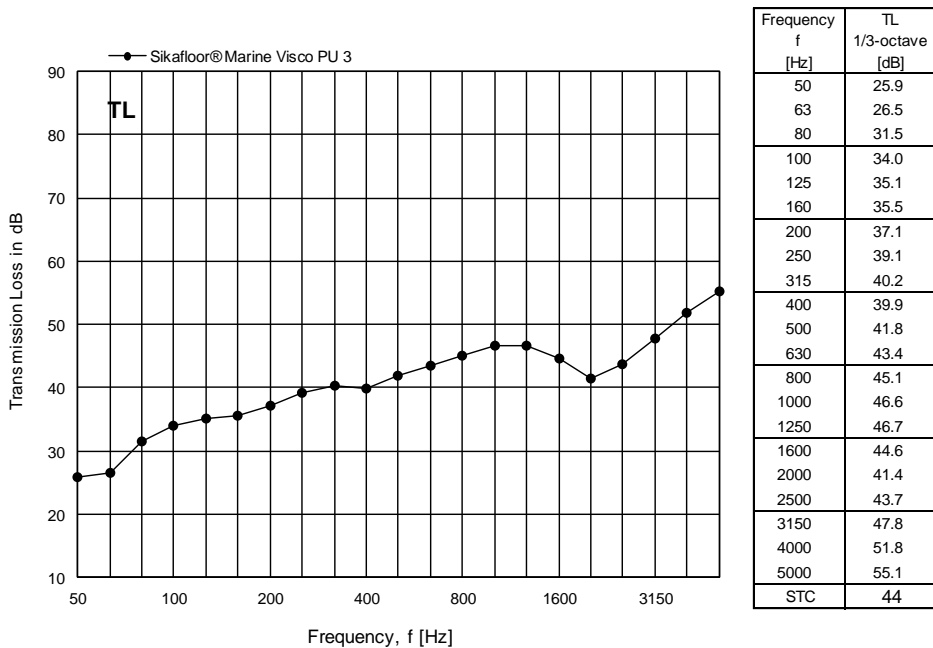
Figure 9 Measured transmission loss TL for Sikafloor® Marine Visco PU 3 expressed in dB per one-third octave frequency band.
