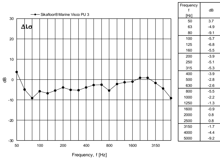
Figure 16 Measured change in radiation efficiency for Sikafloor® Marine Visco PU 3 expressed in dB per one-third octave frequency band.
