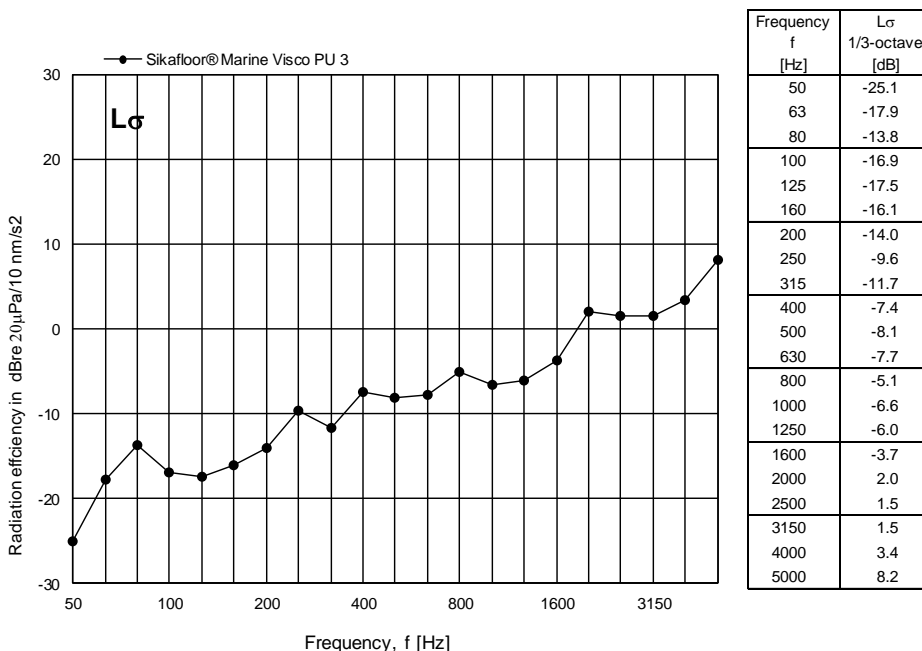
Figure 11 Measured radiation index L_\sigma for Sikafloor® Marine Visco PU 3 expressed in dB per one-third octave frequency band.
