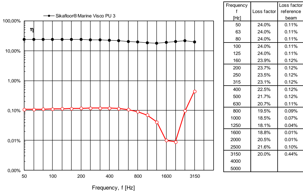
Figure 12 Measured loss factor for test beam applied with constrained damped construction type Sikafloor® Marine Visco PU 3 in % per one-third octave frequency band. For comparison the results of the measurements on a bare 6 mm steel bar are also shown.
