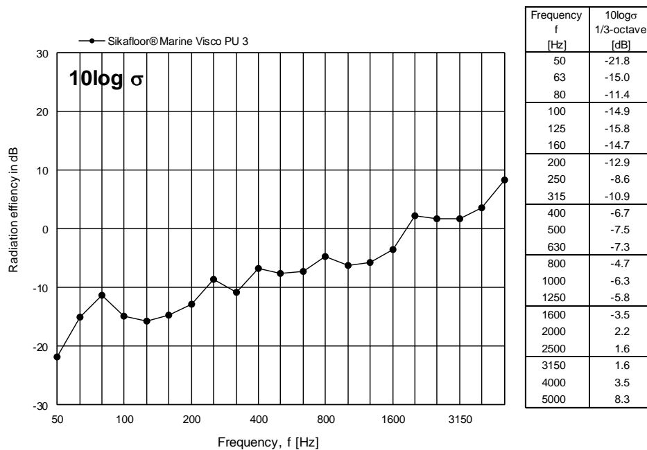
Figure 8 Measured radiation index 10 \log \sigma for Sikafloor® Marine Visco PU 3 expressed in dB per one-third octave frequency band.
