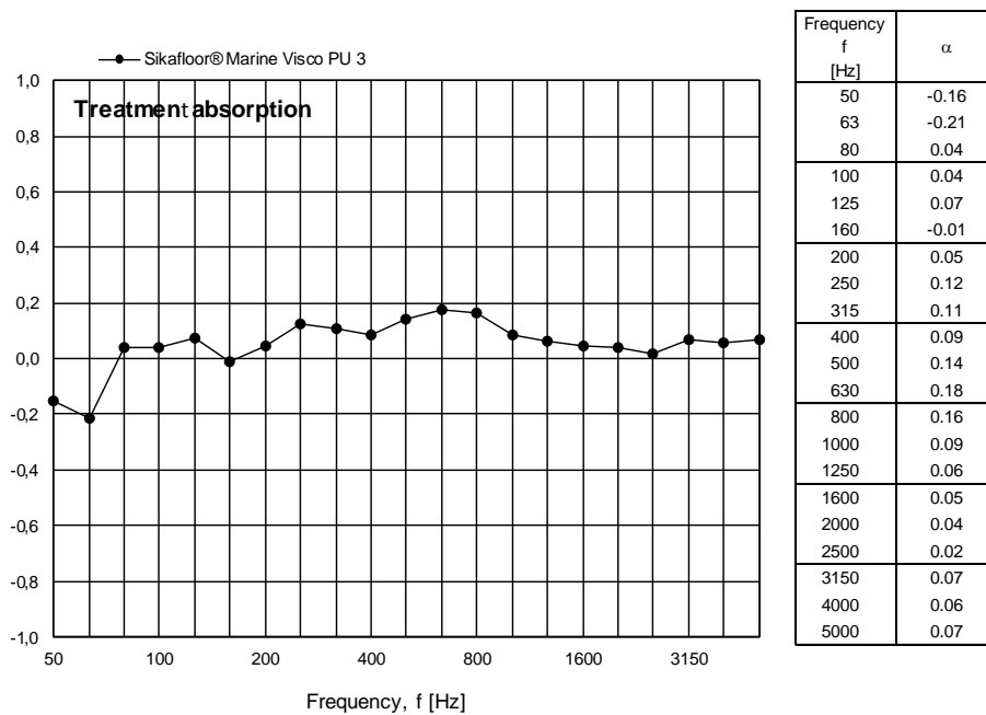
Figure 17 Measured treatment absorption for Sikafloor® Marine Visco PU 3 per one-third octave frequency band.
