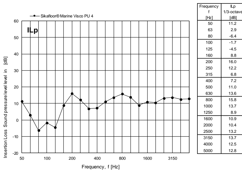
Figure 7 Measured insertion loss IL_p for Sikafloor® Marine Visco Pu 4 expressed in dB per one-third octave frequency band. The insertion loss IL_p refers to the radiated mean sound pressure level in dB re 20 \mu Pa in the receiving room above the floor.
