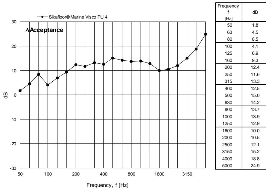
Figure 15 Measured change in acceptance for Sikafloor® Marine Visco PU 4 expressed in dB per one-third octave frequency band.
