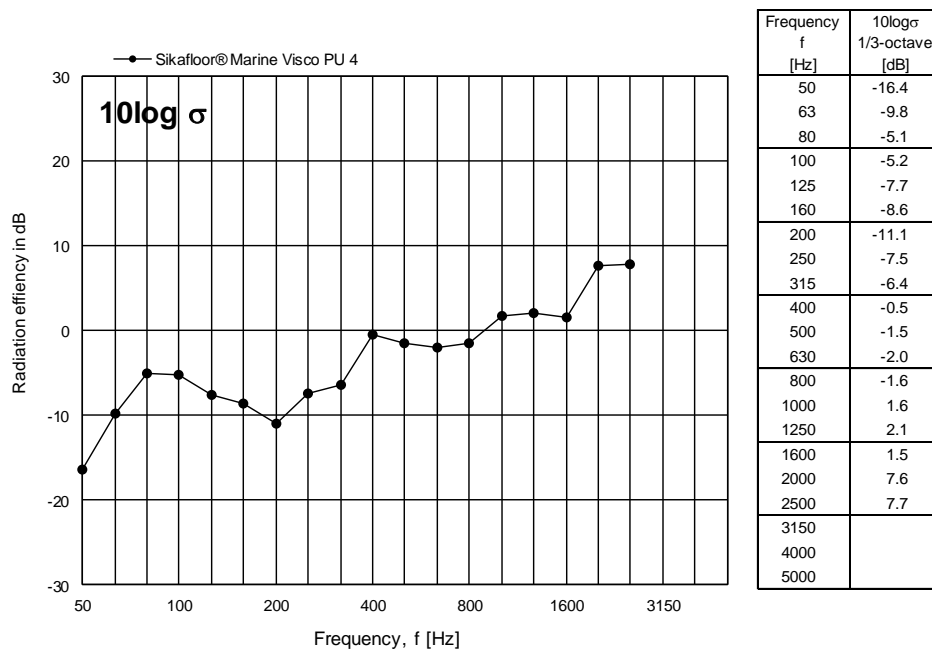
Figure 8 Measured radiation index 10 \log \sigma for Sikafloor® Marine Visco PU 4 expressed in dB per one-third octave frequency band.
