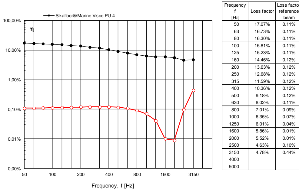
Figure 12 Measured loss factor for test beam applied with constrained damped construction type Sikafloor® Marine Visco PU 4 in % per one-third octave frequency band. For comparison the results of the measurements on a bare 6 mm steel bar are also shown.
