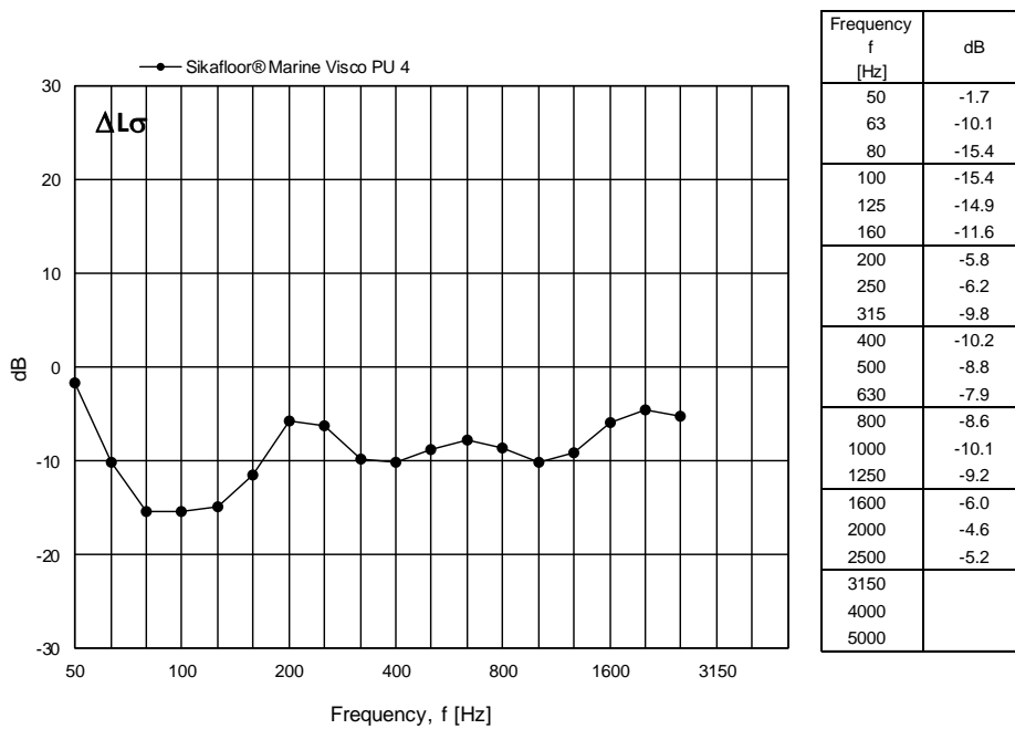
Figure 16 Measured change in radiation efficiency for Sikafloor® Marine Visco PU 4 expressed in dB per one-third octave frequency band.
