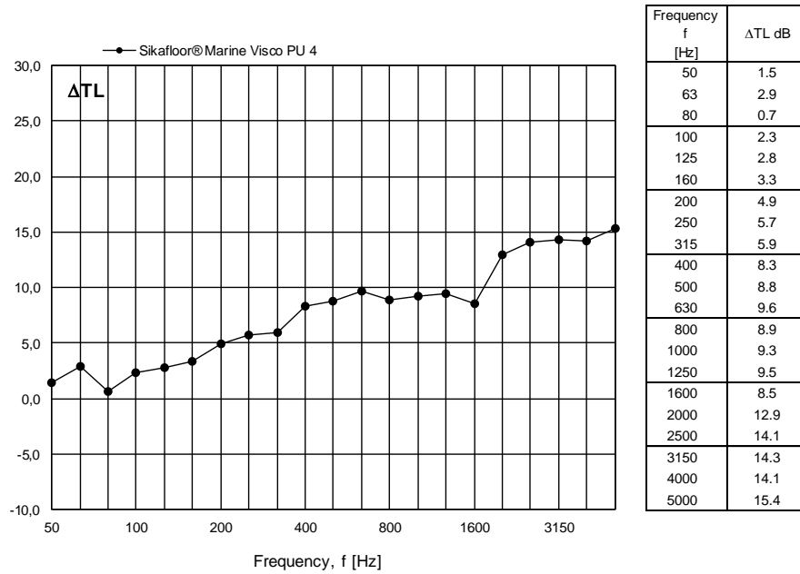
Figure 14 Measured changes in transmission loss TL for Sikafloor® Marine Visco PU 4 expressed in dB per one-third octave frequency band.
