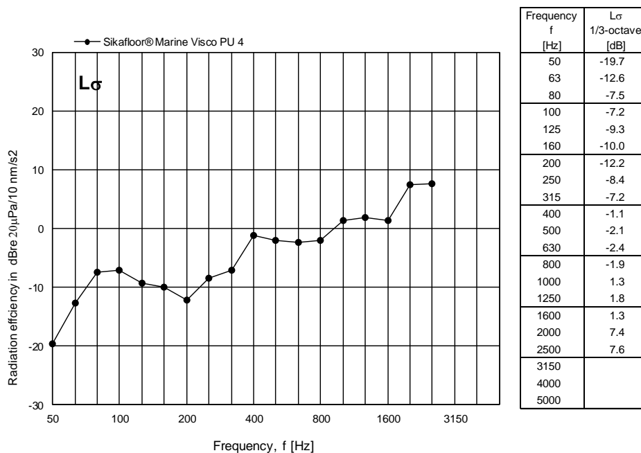
Figure 11 Measured radiation index L_\sigma for Sikafloor® Marine Visco PU 4 expressed in dB per one-third octave frequency band.
