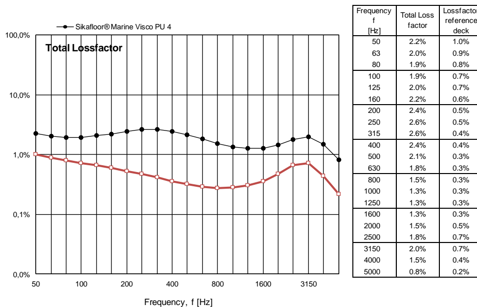
Figure 13 Measured total loss factor for test deck applied with constrained damped construction type Sikafloor® Marine Visco PU 4 in % per one-third octave frequency band. For comparison the results of the measurements on the bare 6 mm steel deck are also shown.
