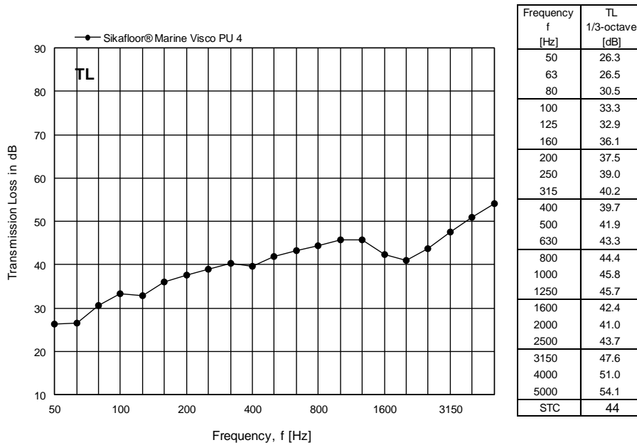
Figure 9 Measured transmission loss TL for Sikafloor® Marine Visco PU 4 expressed in dB per one-third octave frequency band.
