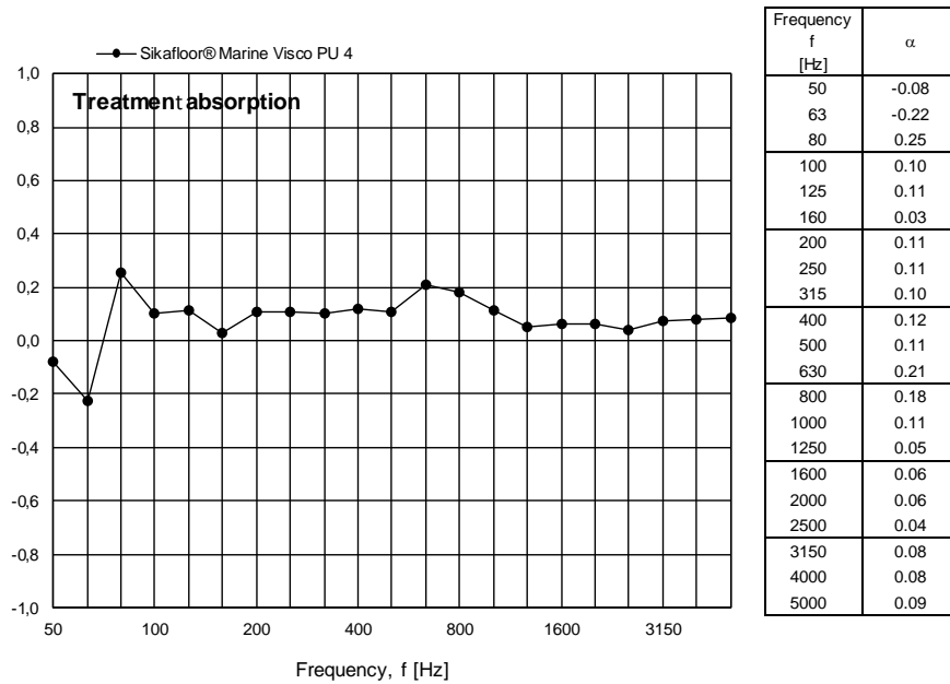
Figure 18 Measured treatment absorption for Sikafloor® Marine Visco PU 4 per one-third octave frequency band.
