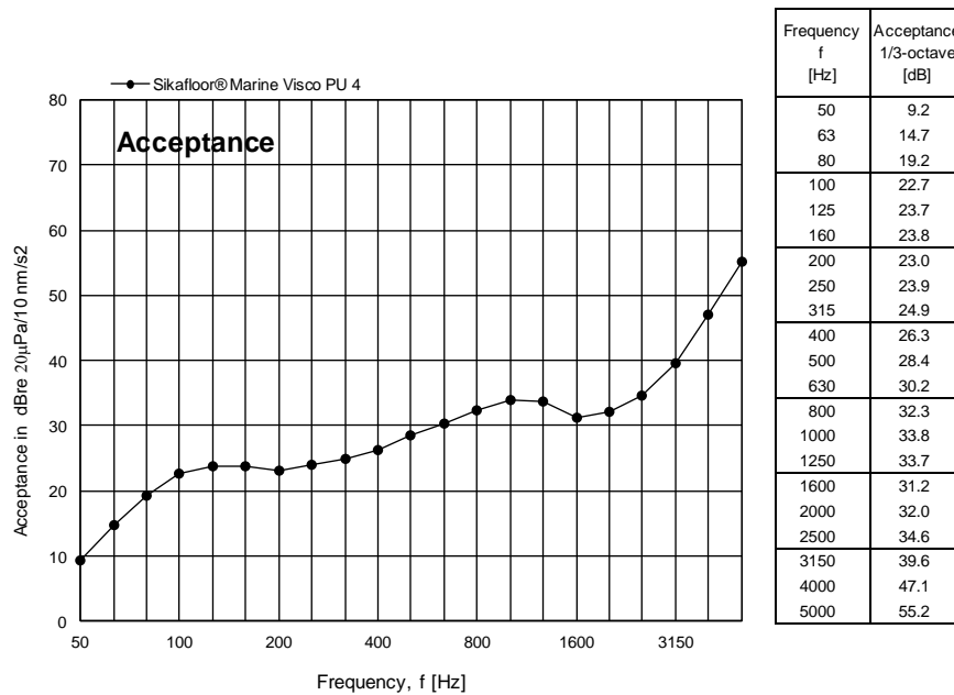
Figure 10 Measured acceptance L_A for Sikafloor® Marine Visco PU 4 expressed in dB per one-third octave frequency band.
