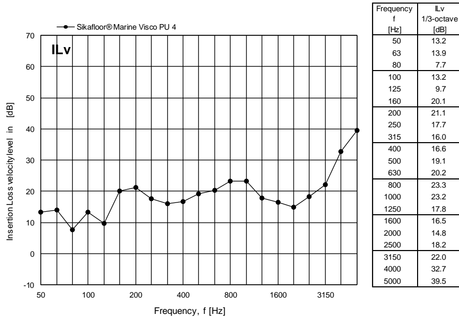
Figure 6 Measured Insertion Loss IL_v for Sikafloor® Marine Visco Pu 4 expressed in dB per one-third octave frequency band. The insertion loss IL_v refers to the mean velocity level in dB re 10 -9 m/s on top of the floor covering.
