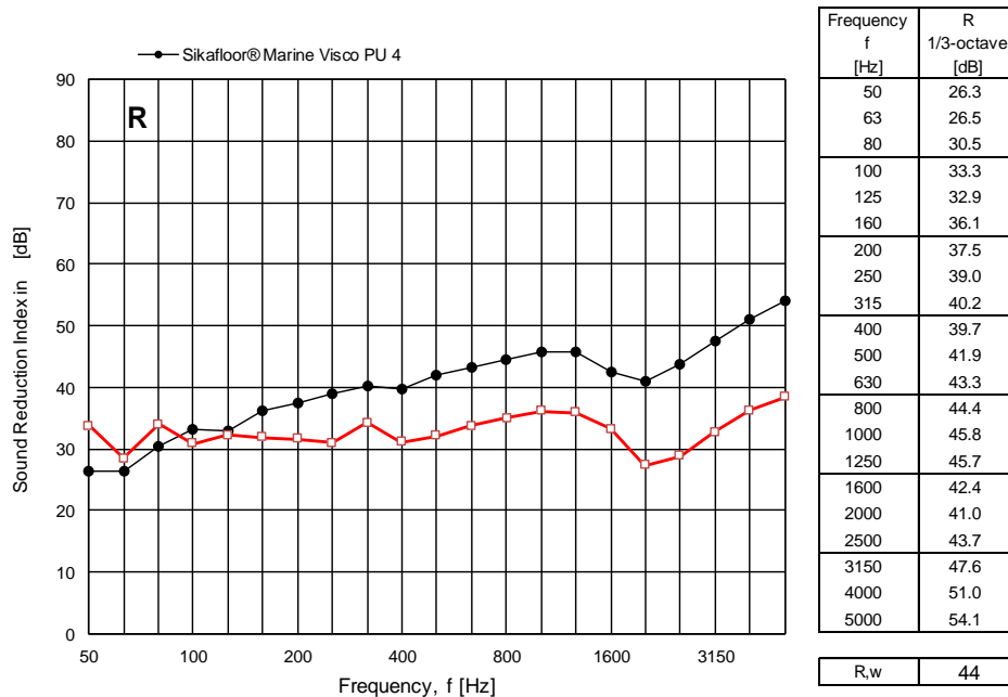
Figure 4 Measured sound reduction index R for the Sikafloor® Marine Visco PU 4 expressed in dB per one-third octave frequency bands. For comparison the results of the measurements on the bare steel deck are also shown.
