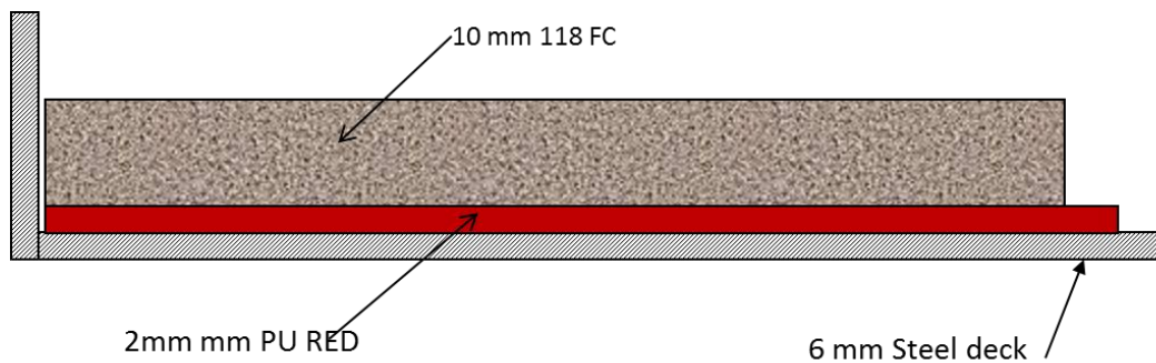
Figure 3 Principle sketch of the test construction.
