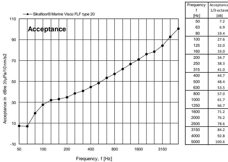
Figure 11 Measured acceptance LA for Sikafloor® Marine Visco FLF type 20 expressed in dB per one-third octave frequency band.
