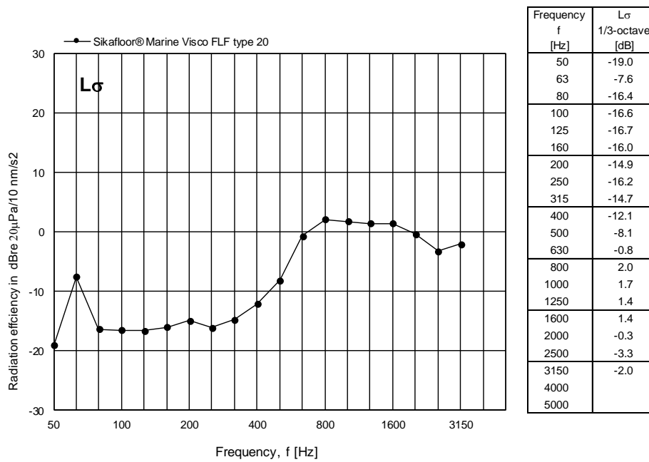
Figure 12 Measured radiation index L_{\sigma} for Sikafloor® Marine Visco FLF type 20 expressed in dB per one-third octave frequency band.
