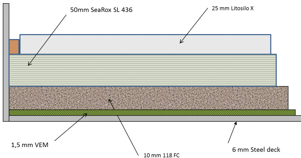
Figure 3 Principle sketch of the test construction.
