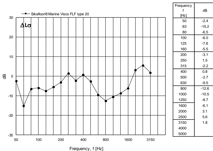
Figure 15 Measured change in radiation efficiency for Sikafloor® Marine Visco FLF type 20 expressed in dB per one-third octave frequency band.
