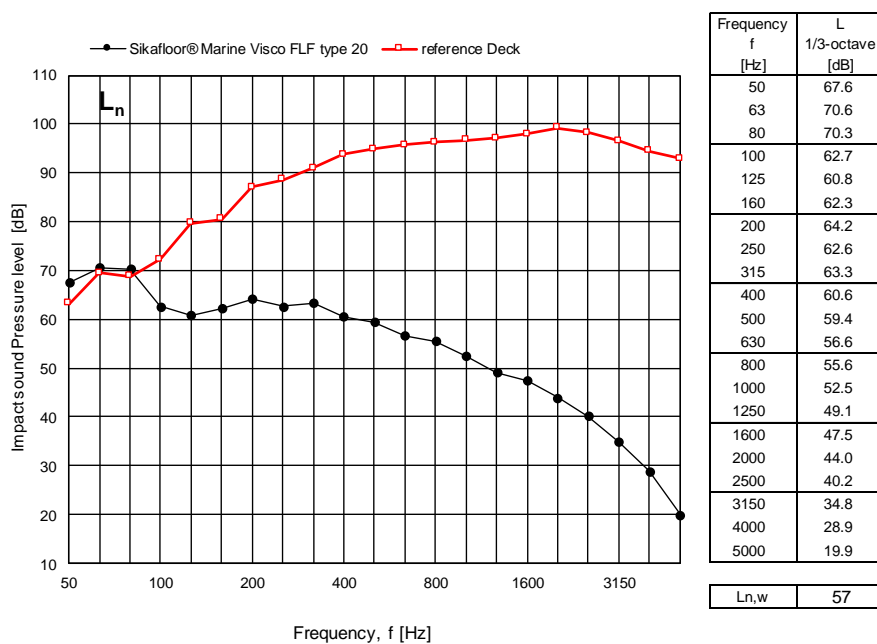
Figure 5 Measured normalized impact sound pressure level L_n for SikaFloor® Marine Visco FLF type 20 expressed in dB re 20 \mu Pa per one-third octave frequency band. For comparison the results of the measurements on the bare steel deck are also shown.
