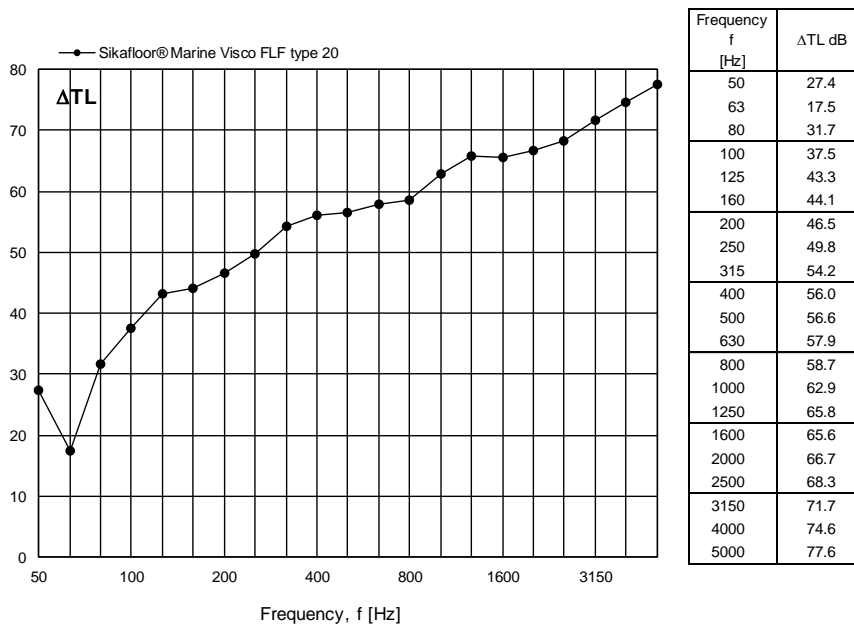
Figure 13 Measured changes in transmission loss TL for Sikafloor® Marine Visco FLF type 20 expressed in dB per one-third octave frequency band.
