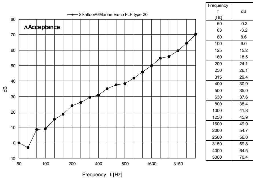
Figure 14 Measured change in acceptance for Sikafloor® Marine Visco FLF type 20 expressed in dB per one-third octave frequency band.
