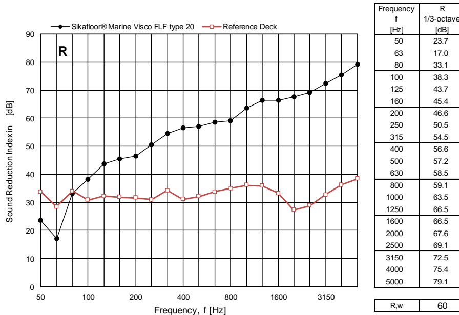
Figure 4 Measured sound reduction index R for the SikaFloor® Marine Visco FLF type 20 expressed in dB per one-third octave frequency bands. For comparison the results of the measurements on the bare steel deck are also shown.
