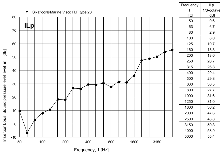
Figure 8 Measured insertion loss IL_p for Sikafloor® Marine Visco FLF type 20 expressed in dB per one-third octave frequency band. The insertion loss IL_p refers to the radiated mean sound pressure level in dB re 20 \mu Pa in the receiving room above the floor.
