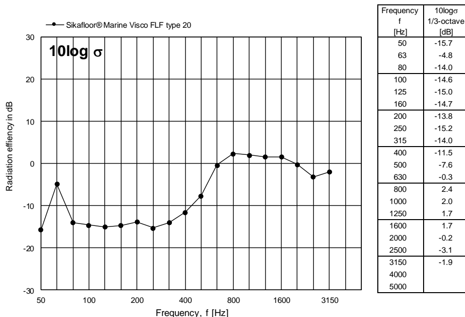
Figure 9 Measured radiation index 10 \log \sigma for Sikafloor® Marine Visco FLF type 20 expressed in dB per one-third octave frequency band.
