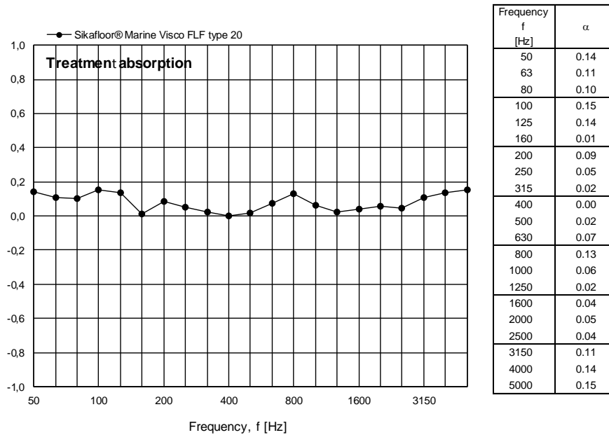
Figure 16 Measured treatment absorption for Sikafloor® Marine Visco FLF type 20 per one-third octave frequency band.
