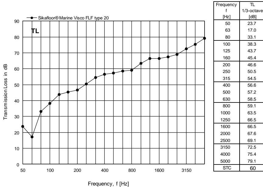
Figure 10 Measured transmission loss TL for Sikafloor® Marine Visco FLF type 20 expressed in dB per one-third octave frequency band.
