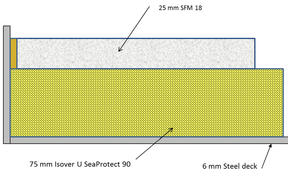
Figure 3 Principle sketch of the test construction.
