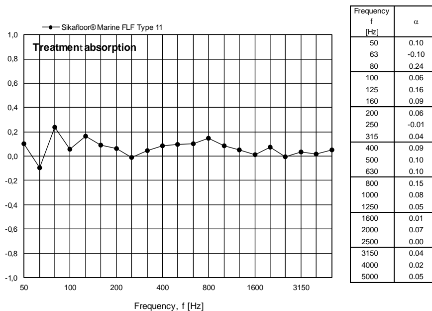
Figure 16 Measured treatment absorption for Sikafloor® Marine FLF Type 11 per one-third octave frequency band.
