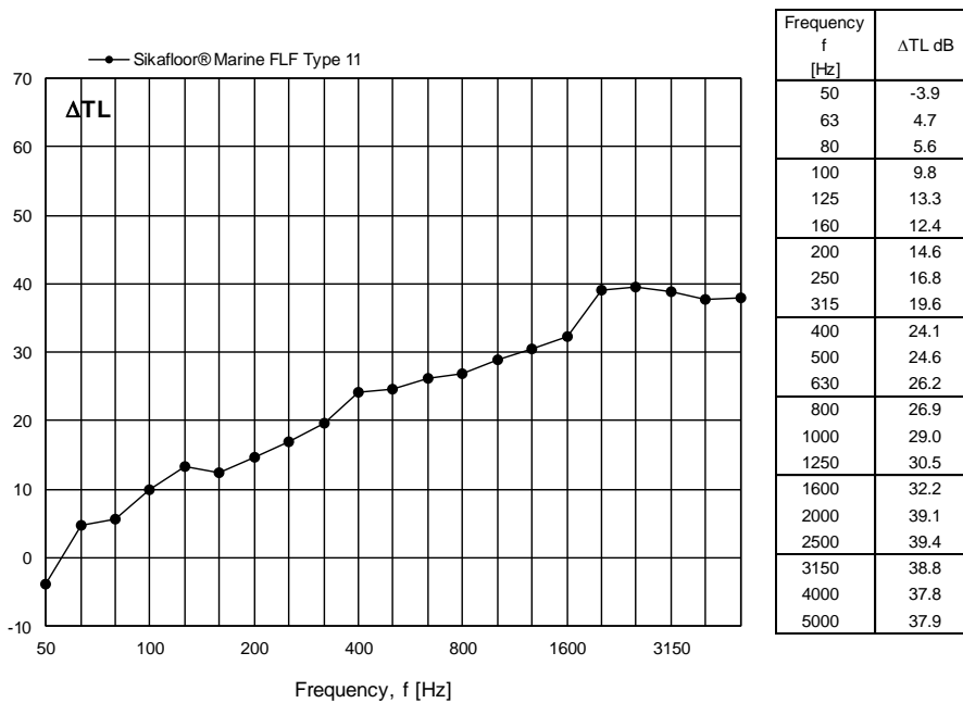
Figure 13 Measured changes in transmission loss TL for Sikafloor® Marine FLF Type 11 expressed in dB per one-third octave frequency band.
