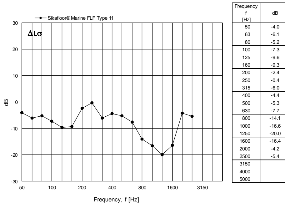
Figure 15 Measured change in radiation efficiency for Sikafloor® Marine FLF Type 11 expressed in dB per one-third octave frequency band.
