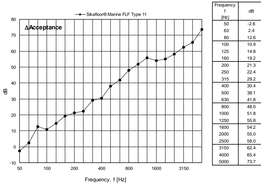
Figure 14 Measured change in acceptance for Sikafloor® Marine FLF Type 11 expressed in dB per one-third octave frequency band.
