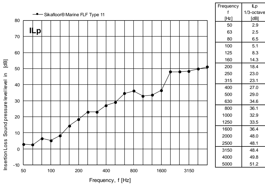
Figure 8 Measured insertion loss IL_p for Sikafloor® Marine FLF Type 11 expressed in dB per one-third octave frequency band. The insertion loss IL_p refers to the radiated mean sound pressure level in dB re 20 \mu Pa in the receiving room above the floor.
