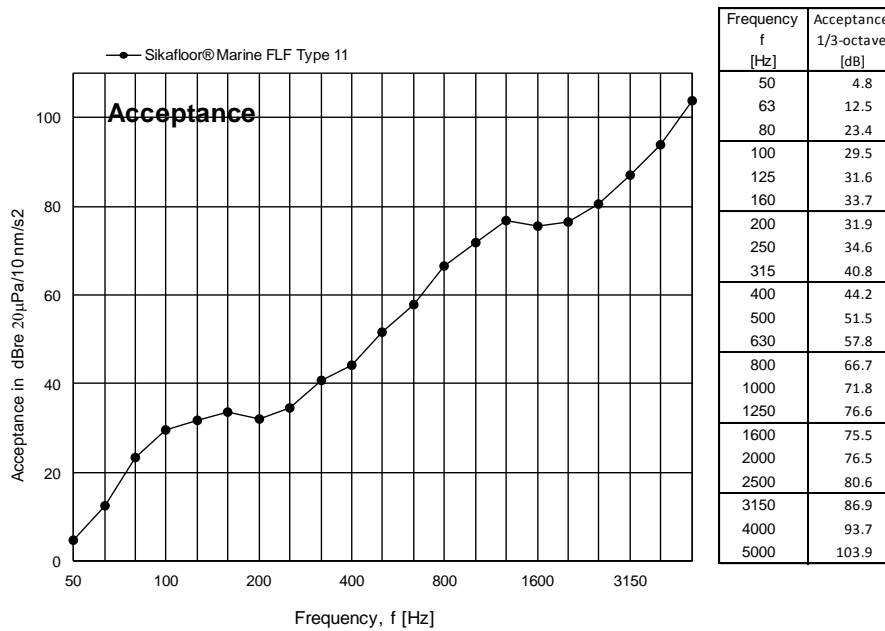
Figure 11 Measured acceptance LA for Sikafloor® Marine FLF Type 11 expressed in dB per one-third octave frequency band.
