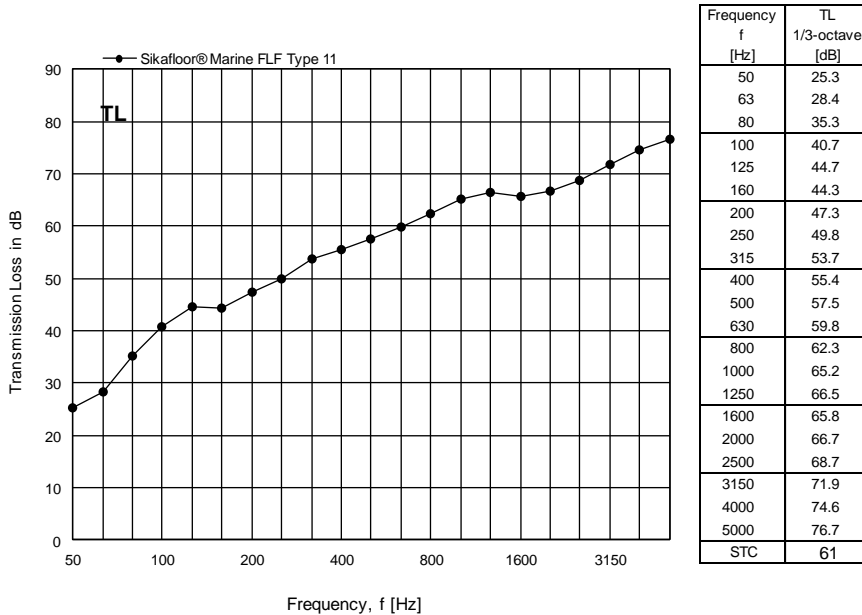
Figure 10 Measured transmission loss TL for Sikafloor® Marine FLF Type 11 expressed in dB per one-third octave frequency band.
