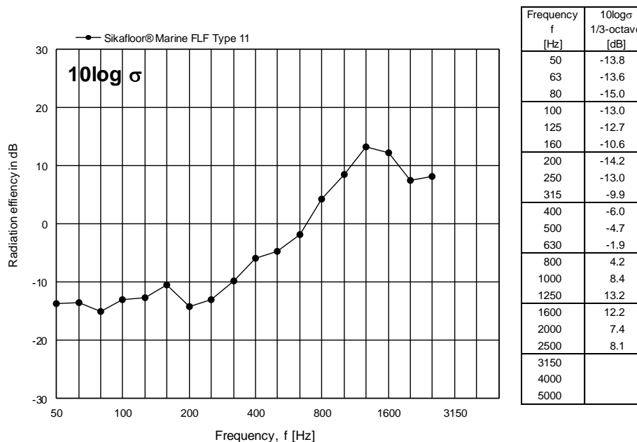
Figure 9 Measured radiation index 10 \log \sigma for Sikafloor® Marine FLF Type 11 expressed in dB per one-third octave frequency band.
