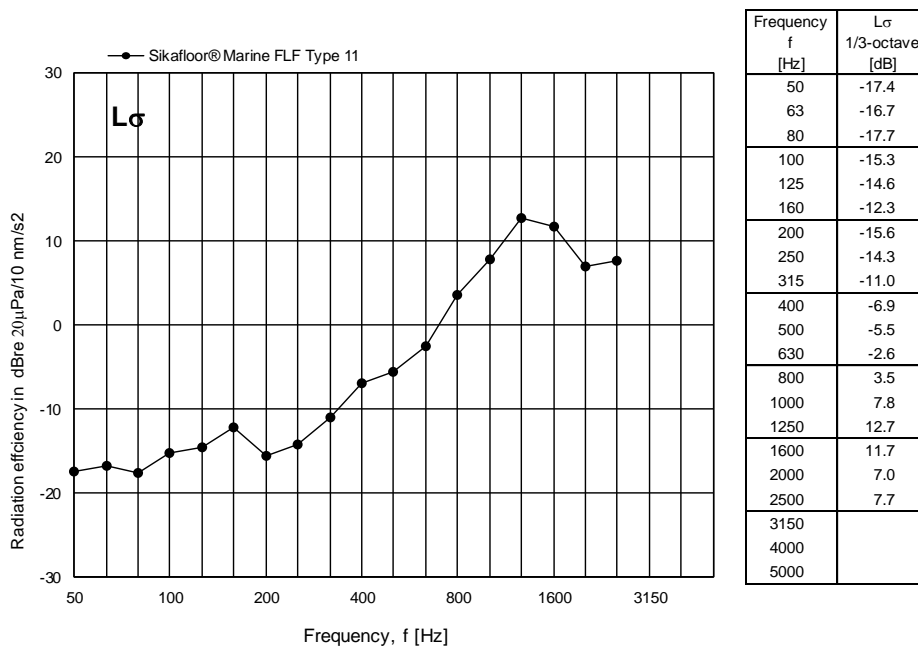
Figure 12 Measured radiation index L_{\sigma} for Sikafloor® Marine FLF Type 11 expressed in dB per one-third octave frequency band.
