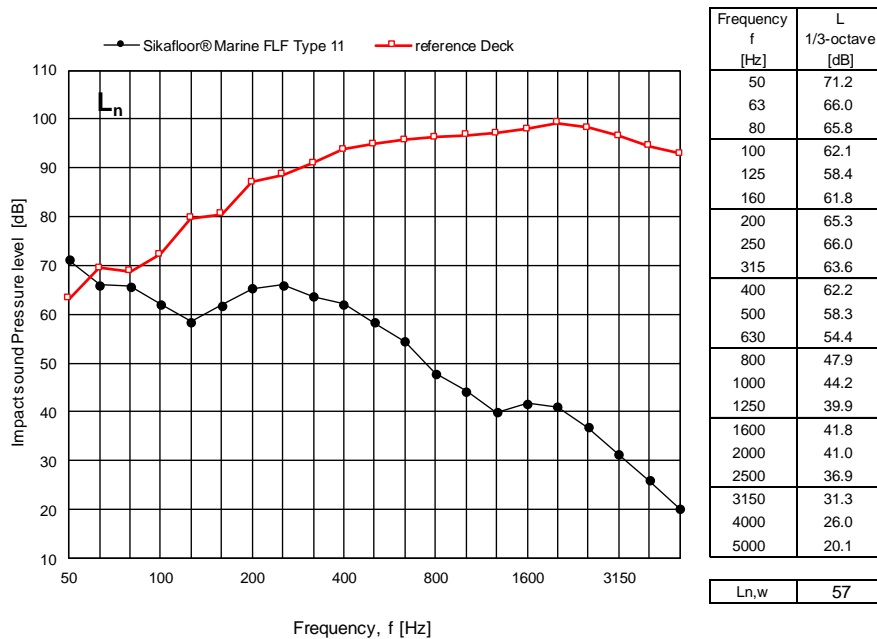
Figure 5 Measured normalized impact sound pressure level L_n for Sikafloor® Marine FLF Type 11 expressed in dB re 20 \mu Pa per one-third octave frequency band. For comparison the results of the measurements on the bare steel deck are also shown.
