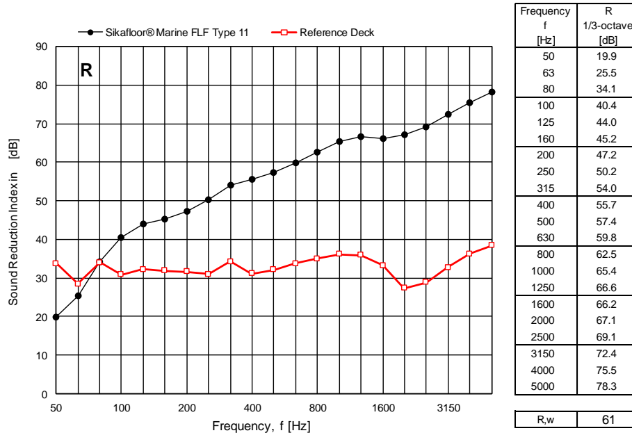
Figure 4 Measured sound reduction index R for the Sikafloor® Marine FLF Type 11 expressed in dB per one-third octave frequency bands. For comparison the results of the measurements on the bare steel deck are also shown.
