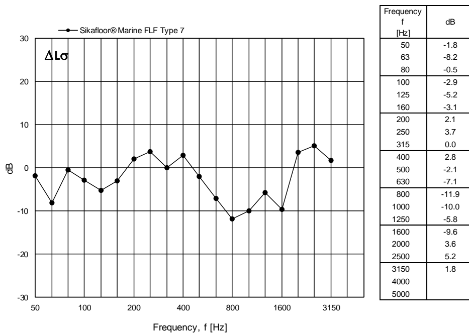
Figure 15 Measured change in radiation efficiency for Sikafloor® Marine FLF Type 7 expressed in dB per one-third octave frequency band.
