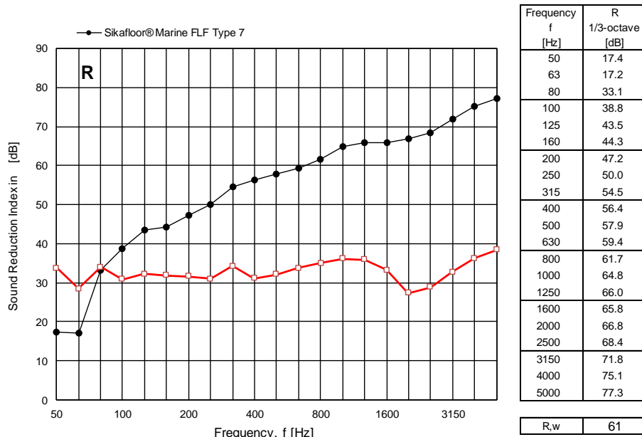
Figure 4 Measured sound reduction index R for the Sikafloor® Marine FLF Type 7 expressed in dB per one-third octave frequency bands. For comparison the results of the measurements on the bare steel deck are also shown.
