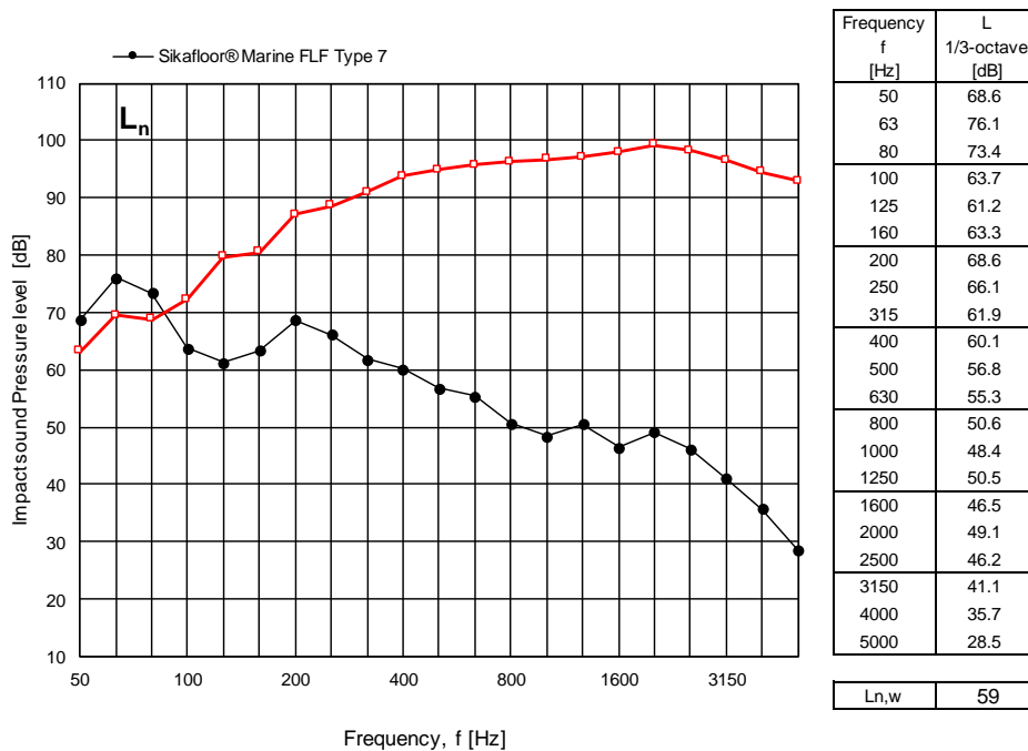
Figure 5 Measured normalized impact sound pressure level L_n for Sikafloor® Marine FLF Type 7 expressed in dB re 20 \mu Pa per one-third octave frequency band. For comparison the results of the measurements on the bare steel deck are also shown.
