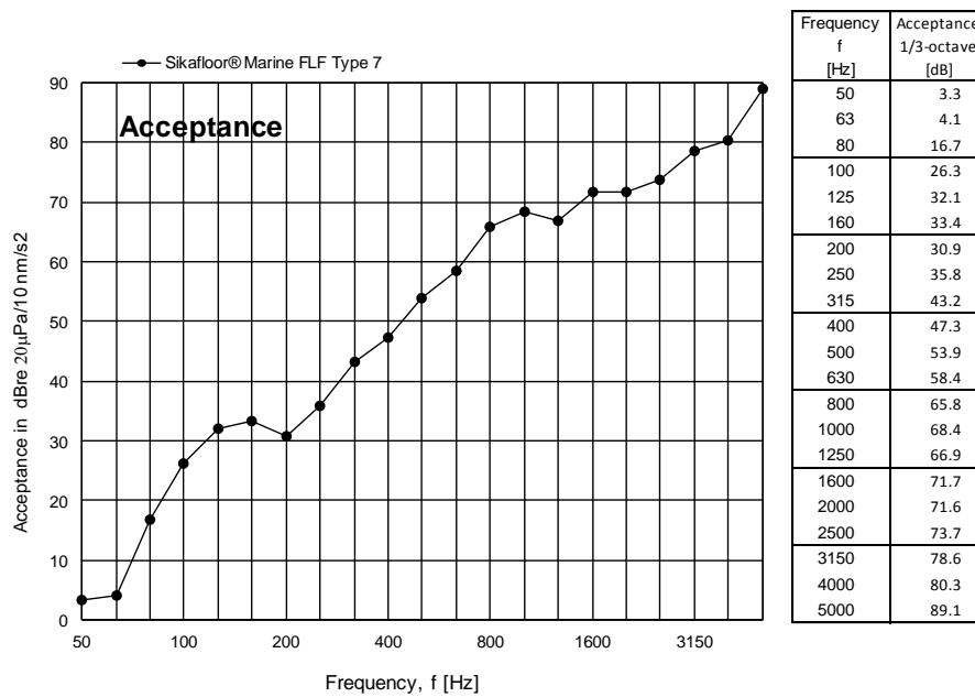
Figure 11 Measured acceptance LA for Sikafloor® Marine FLF Type 7 expressed in dB per one-third octave frequency band.
