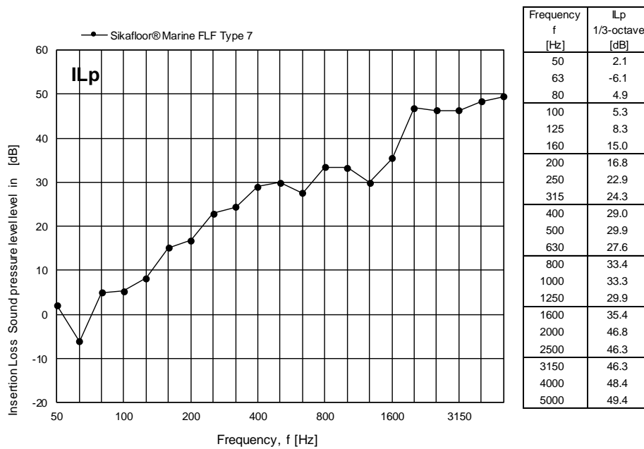
Figure 8 Measured insertion loss IL_p for Sikafloor® Marine FLF Type 7 expressed in dB per one-third octave frequency band. The insertion loss IL_p refers to the radiated mean sound pressure level in dB re 20 \mu Pa in the receiving room above the floor.
