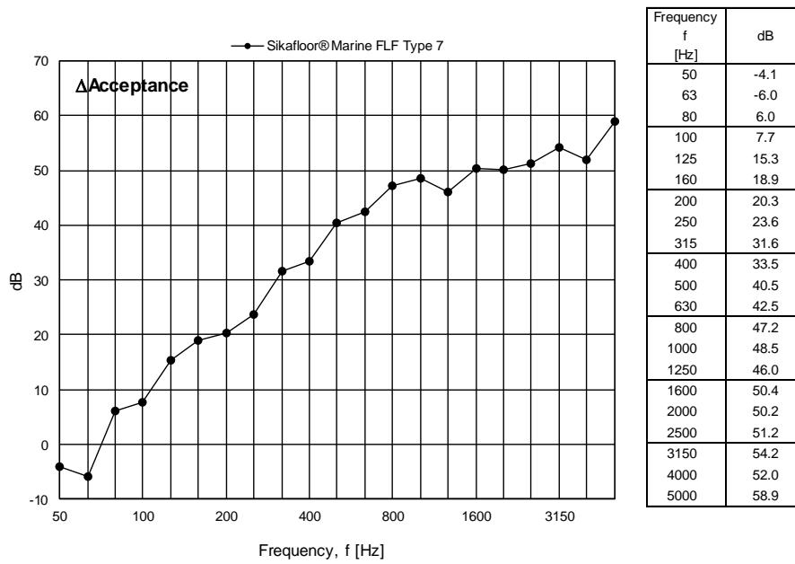
Figure 14 Measured change in acceptance for Sikafloor® Marine FLF Type 7 expressed in dB per one-third octave frequency band.
