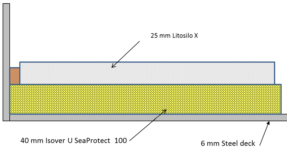
Figure 3 Principle sketch of the test construction.
