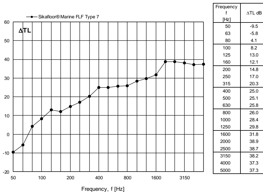
Figure 13 Measured changes in transmission loss TL for Sikafloor® Marine FLF Type 7 expressed in dB per one-third octave frequency band.
