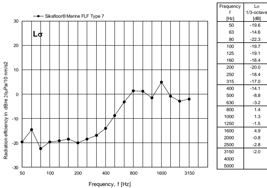
Figure 12 Measured radiation index L_{\sigma} for Sikafloor® Marine FLF Type 7 expressed in dB per one-third octave frequency band.
