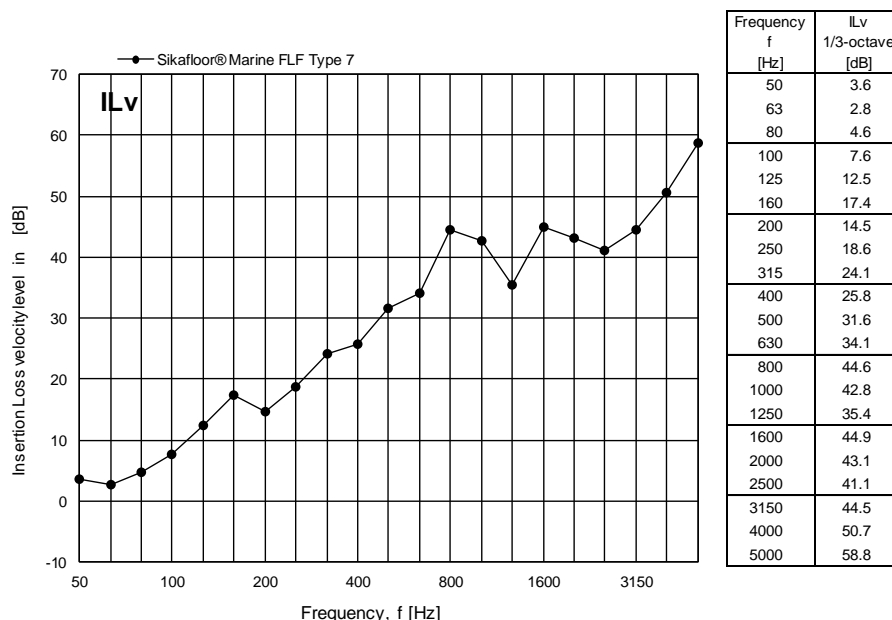
Figure 6 Measured Insertion Loss IL_v for Sikafloor® Marine FLF Type 7 expressed in dB per one-third octave frequency band. The insertion loss IL_v refers to the mean velocity level in dB re 10 -9 m/s on top of the floor covering.
