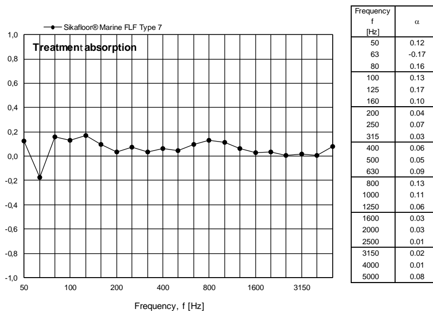
Figure 16 Measured treatment absorption for Sika floor® Marine FLF Type 7 per one-third octave frequency band.
