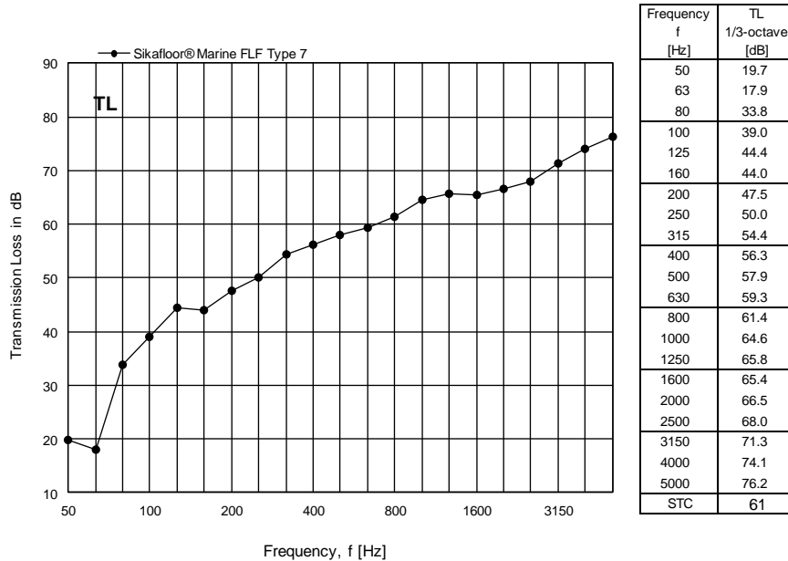
Figure 10 Measured transmission loss TL for Sikafloor® Marine FLF Type 7 expressed in dB per one-third octave frequency band.
