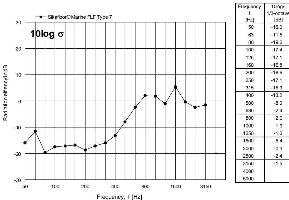
Figure 9 Measured radiation index 10 \log \sigma for Sikafloor® Marine FLF Type 7 expressed in dB per one-third octave frequency band.
