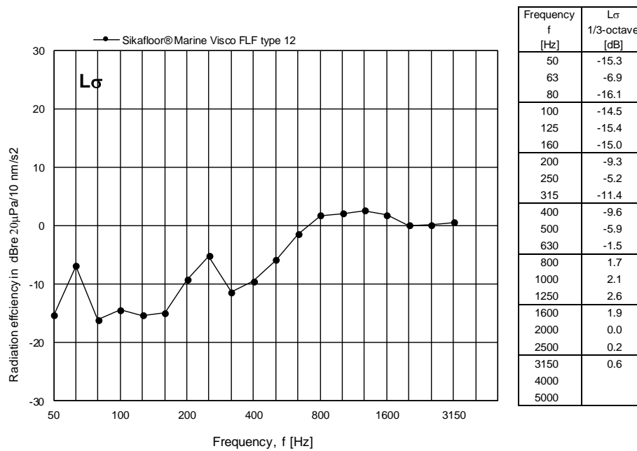
Figure 12 Measured radiation index L_{\sigma} for Sikafloor® Marine Visco FLF type 12 expressed in dB per one-third octave frequency band.
