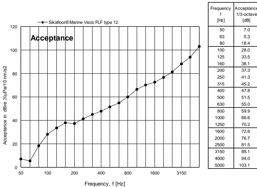
Figure 11 Measured acceptance LA for Sikafloor® Marine Visco FLF type 12 expressed in dB per one-third octave frequency band.
