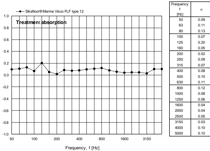
Figure 16 Measured treatment absorption for SikaFloor® Marine Visco FLF type 12 per one-third octave frequency band.
