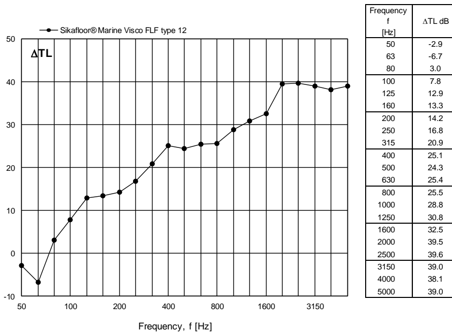
Figure 13 Measured changes in transmission loss TL for Sikafloor® Marine Visco FLF type 12 expressed in dB per one-third octave frequency band.
