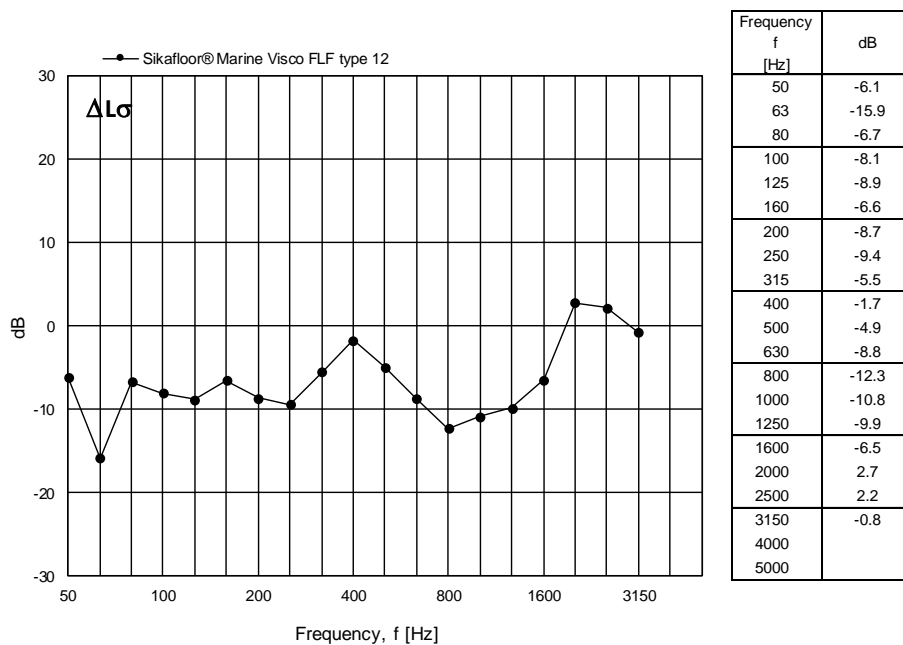
Figure 15 Measured change in radiation efficiency for Sikafloor® Marine Visco FLF type 12 expressed in dB per one-third octave frequency band.
