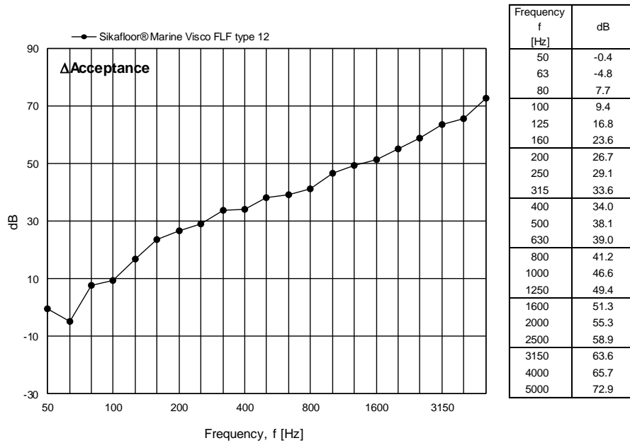
Figure 14 Measured change in acceptance for Sikafloor® Marine Visco FLF type 12 expressed in dB per one-third octave frequency band.
