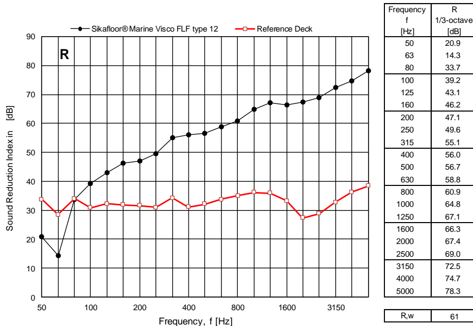
Figure 4 Measured sound reduction index R for the SikaFloor® Marine Visco FLF type 12 expressed in dB per one-third octave frequency bands. For comparison the results of the measurements on the bare steel deck are also shown.
