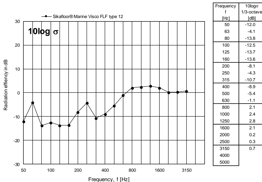
Figure 9 Measured radiation index 10 \log \sigma for Sika floor® Marine Visco FLF type 12 expressed in dB per one-third octave frequency band.
