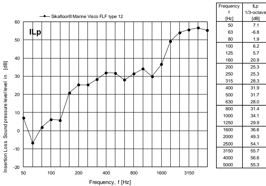
Figure 8 Measured insertion loss IL_p for Sika floor® Marine Visco FLF type 12 expressed in dB per one-third octave frequency band. The insertion loss IL_p refers to the radiated mean sound pressure level in dB re 20 \mu Pa in the receiving room above the floor.
