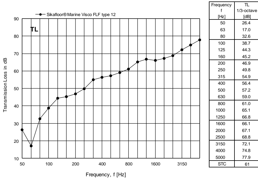
Figure 10 Measured transmission loss TL for Sikafloor® Marine Visco FLF type 12 expressed in dB per one-third octave frequency band.
