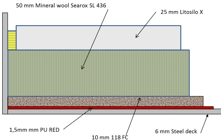
Figure 3 Principle sketch of the test construction.
