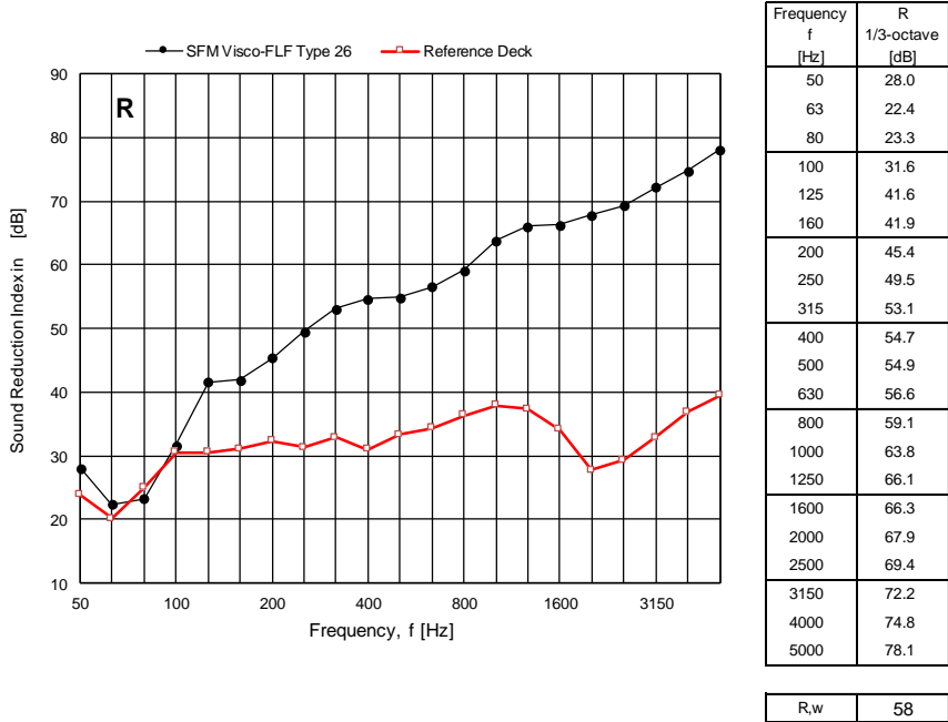
Figure 4 Measured sound reduction index R for the Sikafloor® Marine Visco FLF Type 26 expressed in dB per one-third octave frequency bands. For comparison the results of the measurements on the bare steel deck are also shown.
