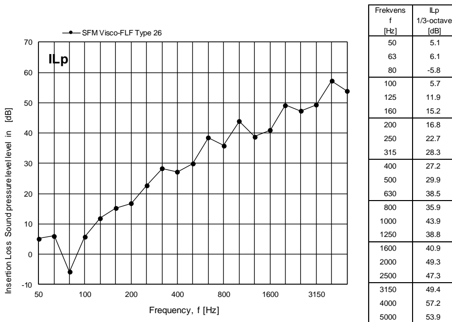
Figure 8 Measured insertion loss IL_p for Sikafloor® Marine Visco FLF Type 26 expressed in dB per one-third octave frequency band. The insertion loss IL_p refers to the radiated mean sound pressure level in dB re 20 \mu Pa in the receiving room above the floor.
