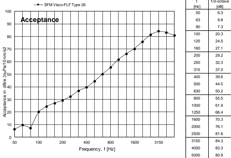
Figure 11 Measured acceptance L A for Sikafloor® Marine Visco FLF Type 26 expressed in dB per one-third octave frequency band.
