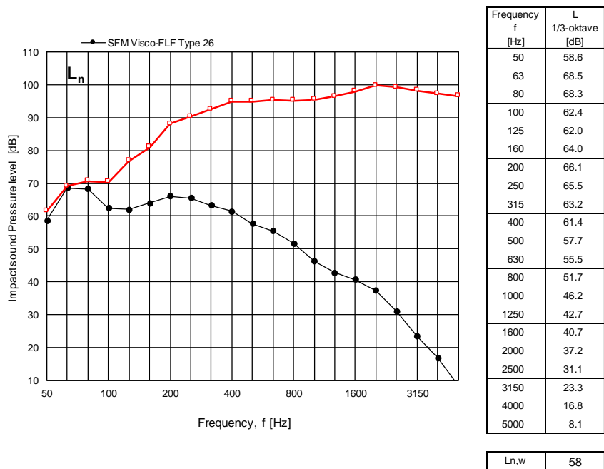
Figure 5 Measured normalized impact sound pressure level L_n for Sikafloor® Marine Visco FLF Type 26 expressed in dB re 20 \mu Pa per one-third octave frequency band. For comparison the results of the measurements on the bare steel deck are also shown.
