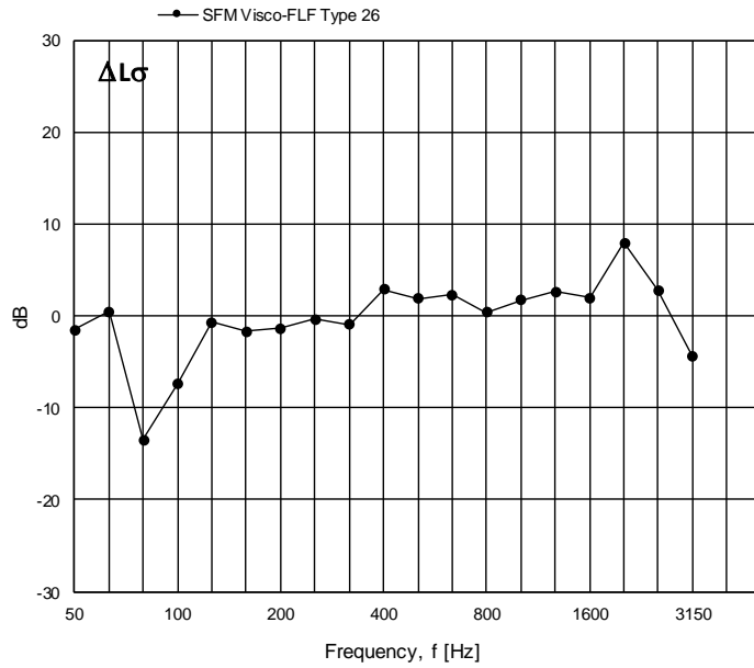
Figure 15 Measured change in radiation efficiency for Sikafloor® Marine Visco FLF Type 26 expressed in dB per one-third octave frequency band.
