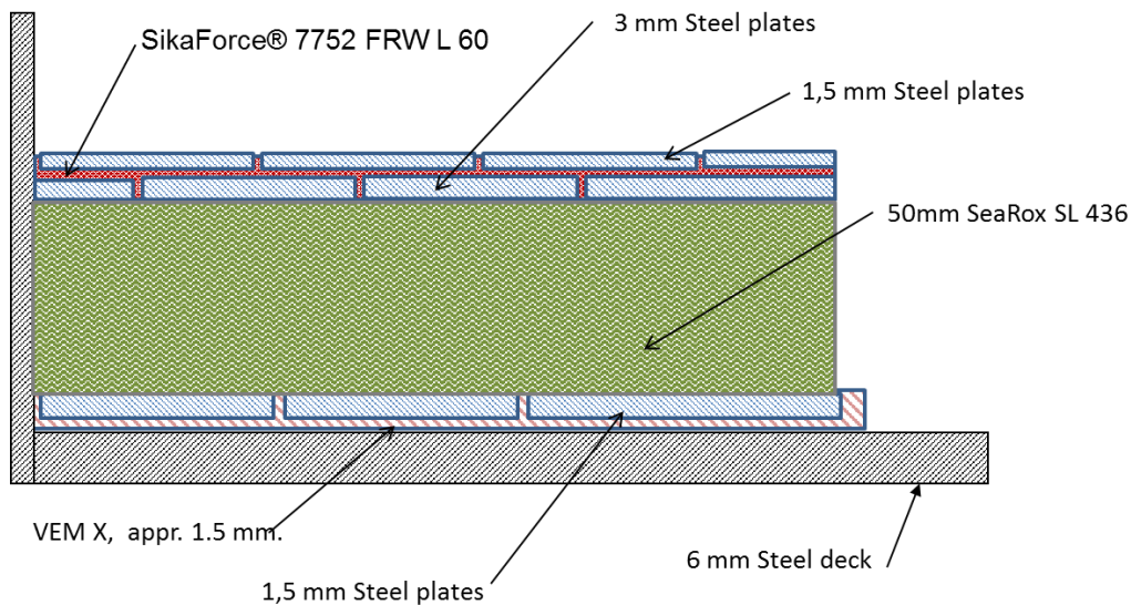
Figure 3 Principle sketch of the test construction.
