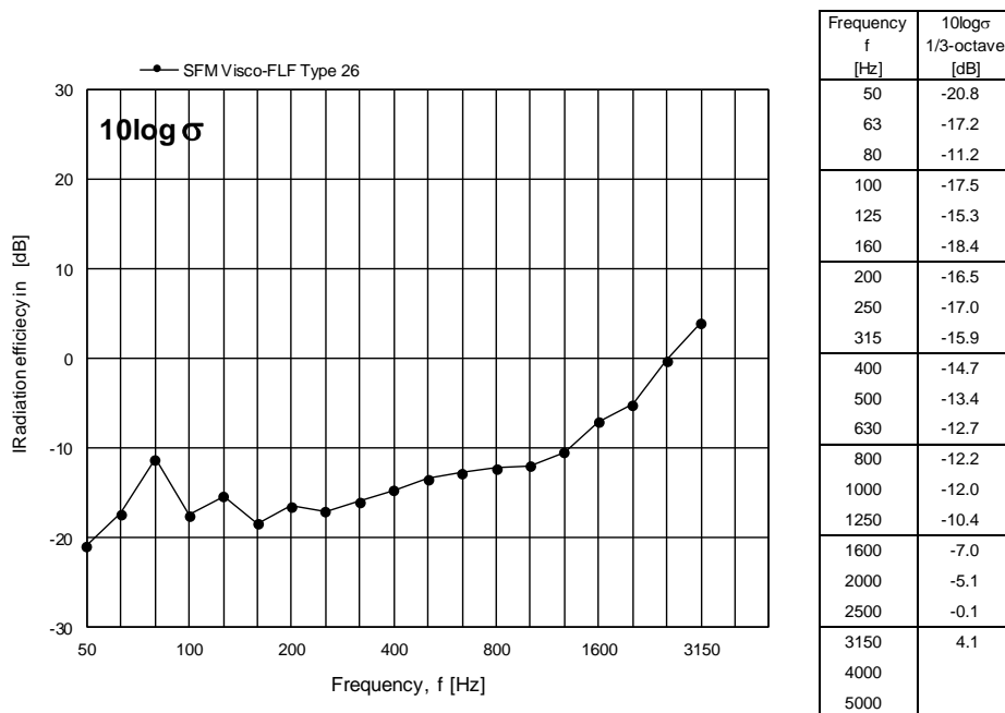
Figure 9 Measured radiation index 10 \log \sigma for Sikafloor® Marine Visco FLF Type 26 expressed in dB per one-third octave frequency band.
