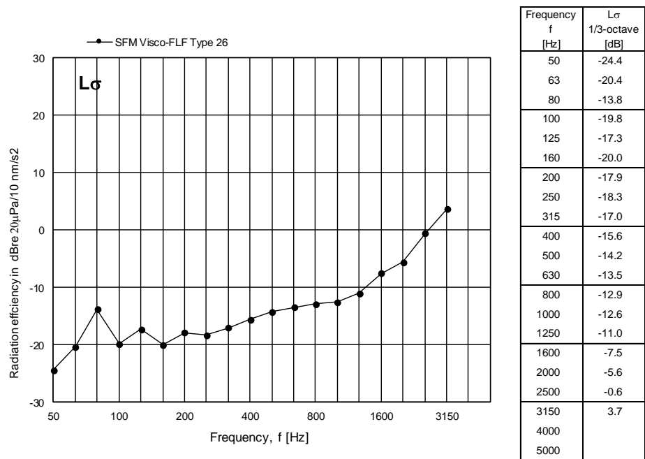
Figure 12 Measured radiation index L_{\sigma} for Sikafloor® Marine Visco FLF Type 26 expressed in dB per one-third octave frequency band.
