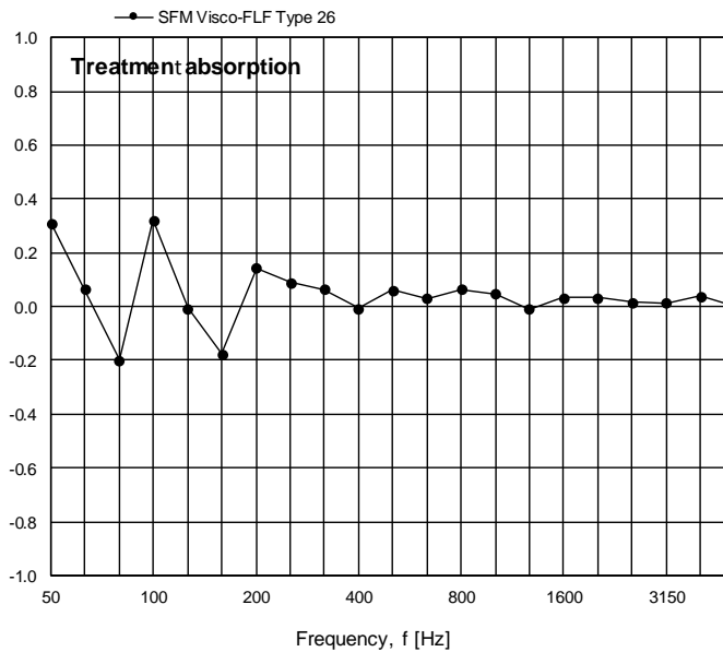
Figure 16 Measured treatment absorption for Sikafloor® Marine Visco FLF Type 26 per one-third octave frequency band.
