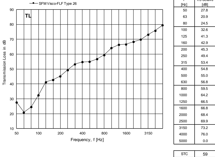
Figure 10 Measured transmission loss TL for Sikafloor® Marine Visco FLF Type 26 expressed in dB per one-third octave frequency band.
