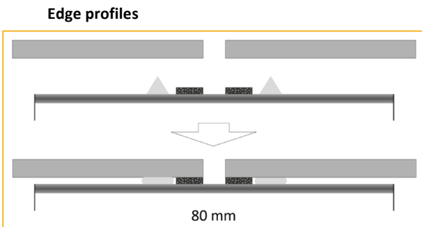
Figure 2: Dilatation taken by the adhesive - edge profile
