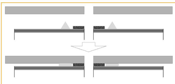
Figure 4: Dilatation taken by the sub-structure - edge profile
