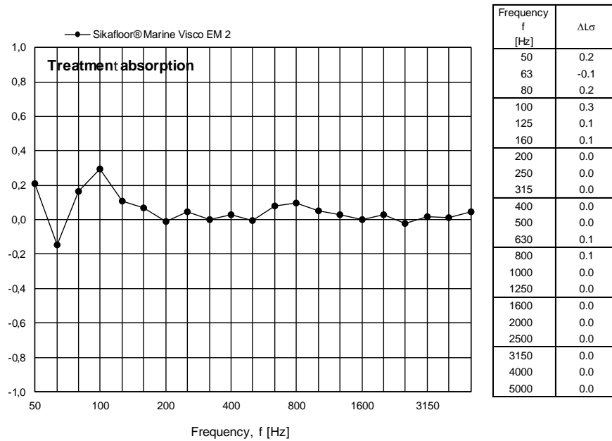
Figure 17 Measured treatment absorption for Sikafloor® Marine Visco EM 2 per one-third octave frequency band.
