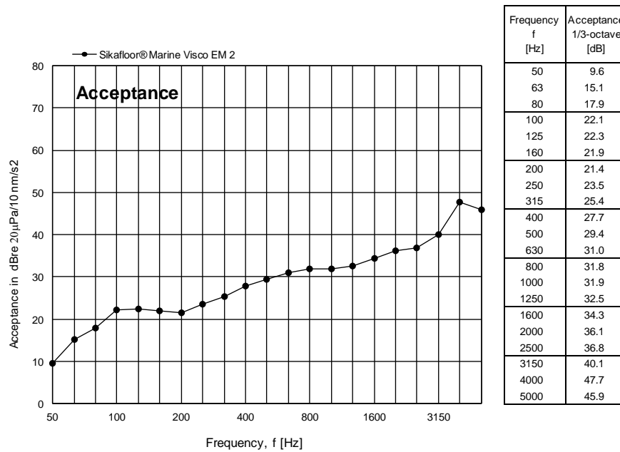
Figure 9 Measured acceptance L_A for Sikafloor® Marine Visco EM 2 expressed in dB per one-third octave frequency band.
