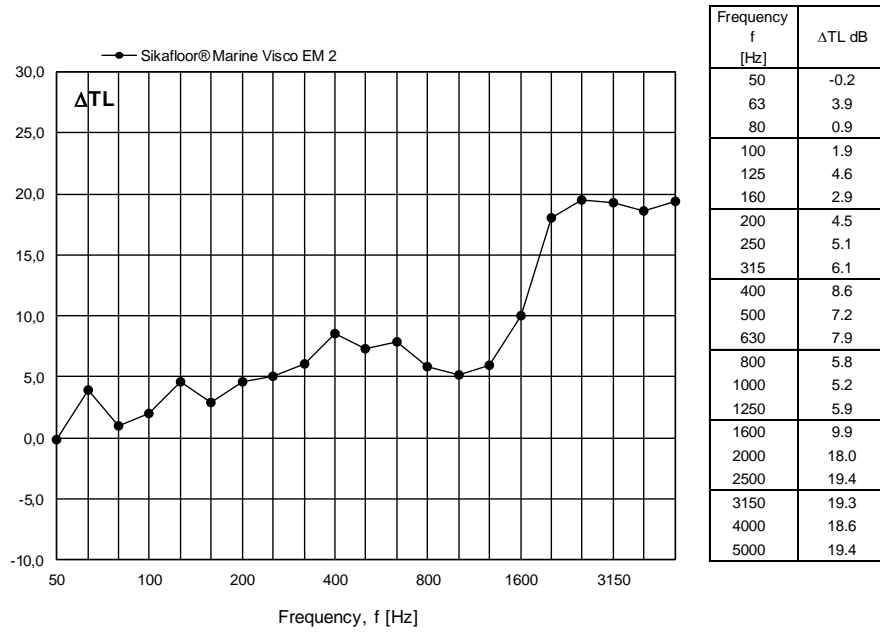
Figure 13 Measured changes in transmission loss TL for Sikafloor® Marine Visco EM 2 expressed in dB per one-third octave frequency band.
