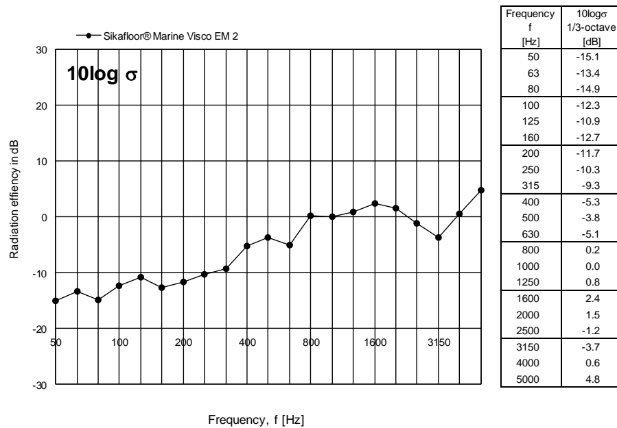
Figure 7 Measured radiation index 10 \log \sigma for Sikafloor® Marine Visco EM 2 expressed in dB per one-third octave frequency band.
