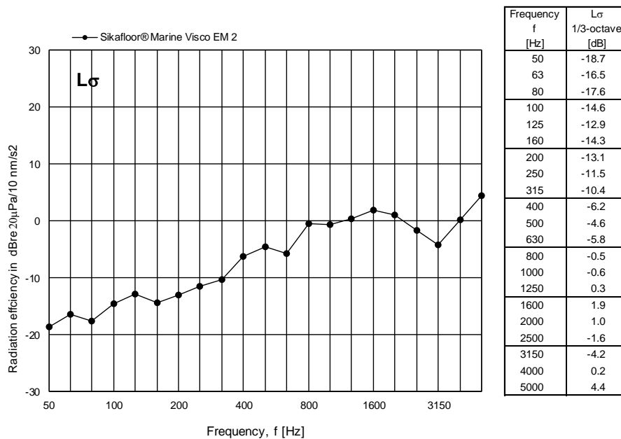
Figure 10 Measured radiation index L_\sigma for Sikafloor® Marine Visco EM 2 expressed in dB per one-third octave frequency band.
