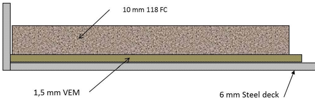
Figure 3 Principle sketch of the test construction.
