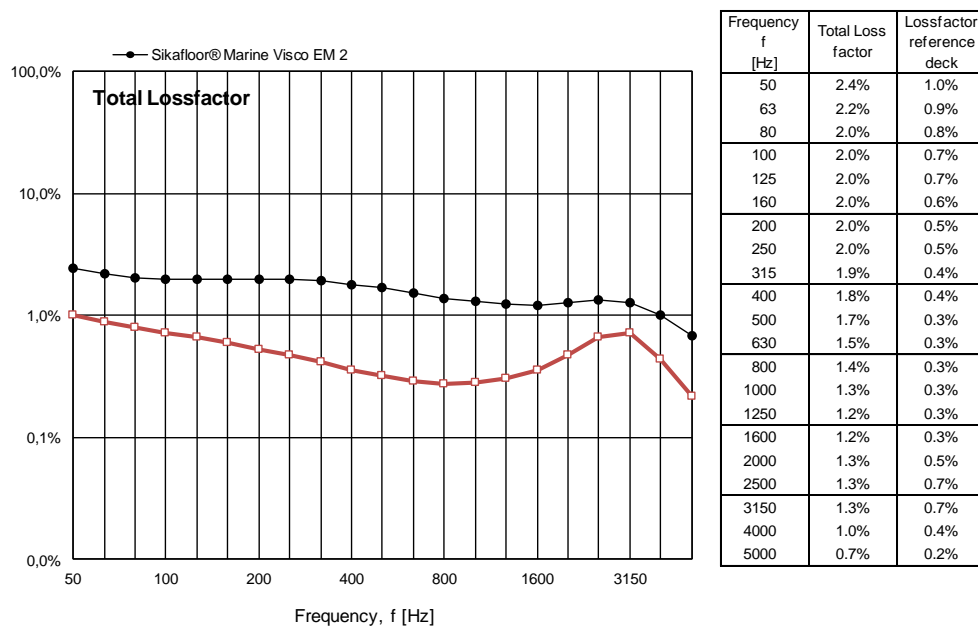
Figure 12 Measured total loss factor for test deck applied with constrained damped construction type Sikafloor® Marine Visco EM 2 in % per one-third octave frequency band. For comparison the results of the measurements on the bare 6 mm steel deck are also shown.
