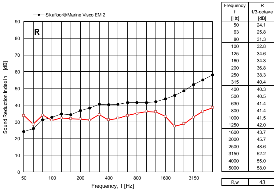
Figure 4 Measured sound reduction index R for the Sikafloor® Marine Visco EM 2 expressed in dB per one-third octave frequency bands. For comparison the results of the measurements on the bare steel deck are also shown.
