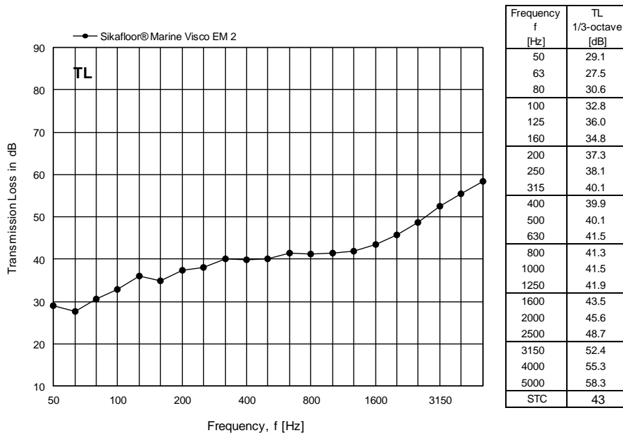
Figure 8 Measured transmission loss TL for Sikafloor® Marine Visco EM 2 expressed in dB per one-third octave frequency band.
