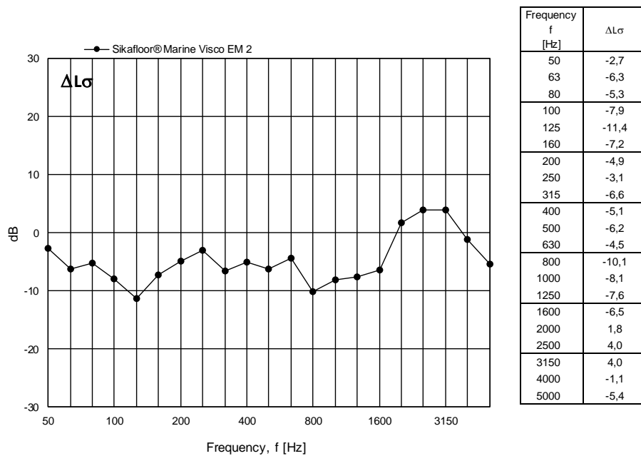
Figure 15 Measured change in radiation efficiency for Sikafloor® Marine Visco EM 2 expressed in dB per one-third octave frequency band.
