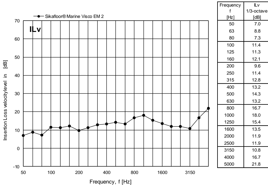
Figure 6 Measured Insertion Loss IL_v for Sikafloor® Marine Visco EM 2 expressed in dB per one-third octave frequency band. The insertion loss IL_v refers to the mean velocity level in dB re 10 -9 m/s on top of the floor covering.
