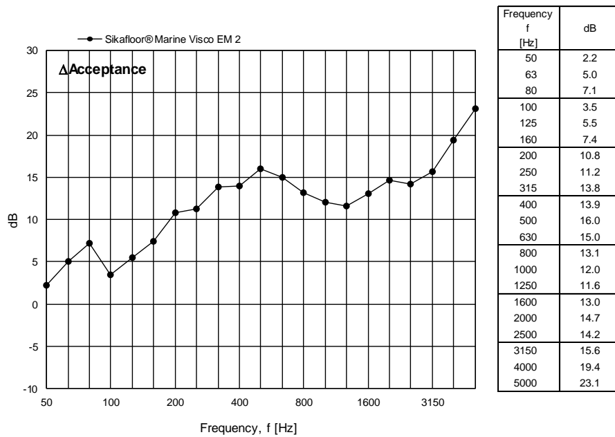
Figure 14 Measured change in acceptance for Sikafloor® Marine Visco EM 2 expressed in dB per one-third octave frequency band.
