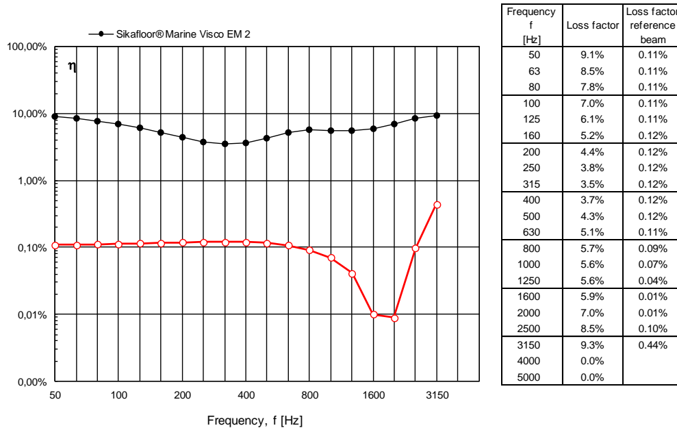
Figure 11 Measured loss factor for test beam applied with constrained damped construction type Sikafloor® Marine Visco EM 2 in % per one-third octave frequency band. For comparison the results of the measurements on a bare 6 mm steel bar are also shown.
