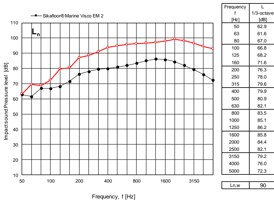
Figure 5 Measured normalized impact sound pressure level L_n for Sikafloor® Marine Visco EM 2 expressed in dB re 20 \mu Pa per one-third octave frequency band. For comparison the results of the measurements on the bare steel deck are also shown.
